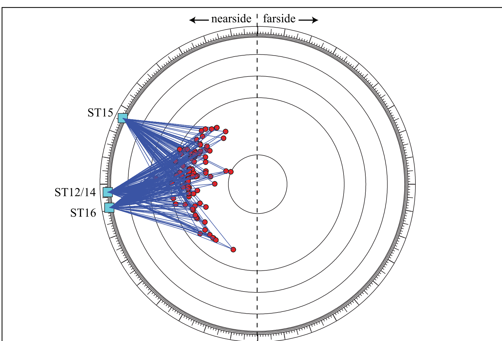
Figure 2: Cross-section showing P-wave coverage from deep moonquakes at the Apollo seismic station locations. Ray paths are projected onto the plane that slices the Moon along the prime meridian. Lateral sampling of rays is small near the surface (limited to the regions directly beneath the Apollo stations), and gradually increases with depth, with the mid-mantle most densely sampled.
