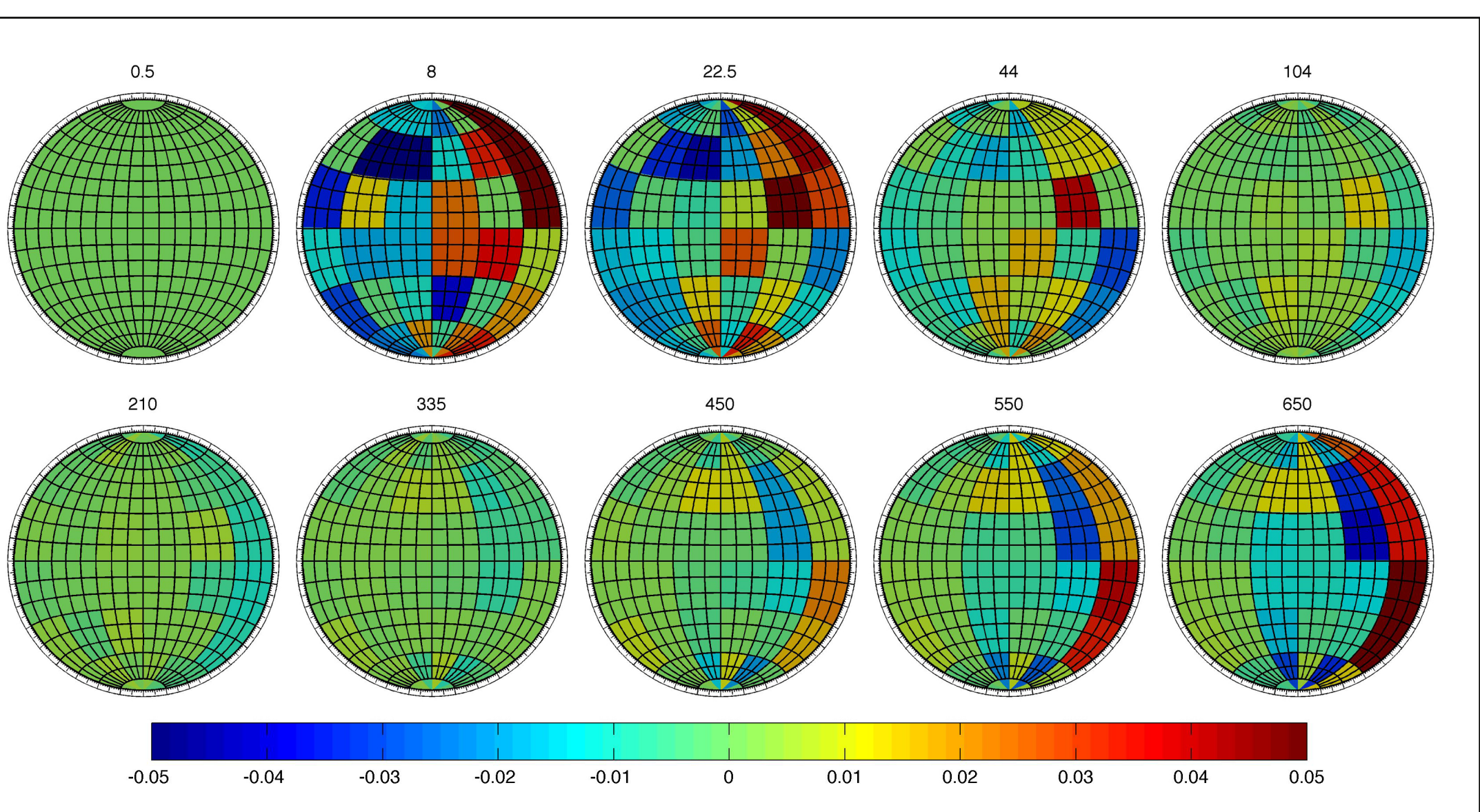
Figure 7: Near-side density anomaly (percent deviation from input model) resulting from the joint inversion, at the modeled layer boundaries. Density blocks are 30° on a side.
