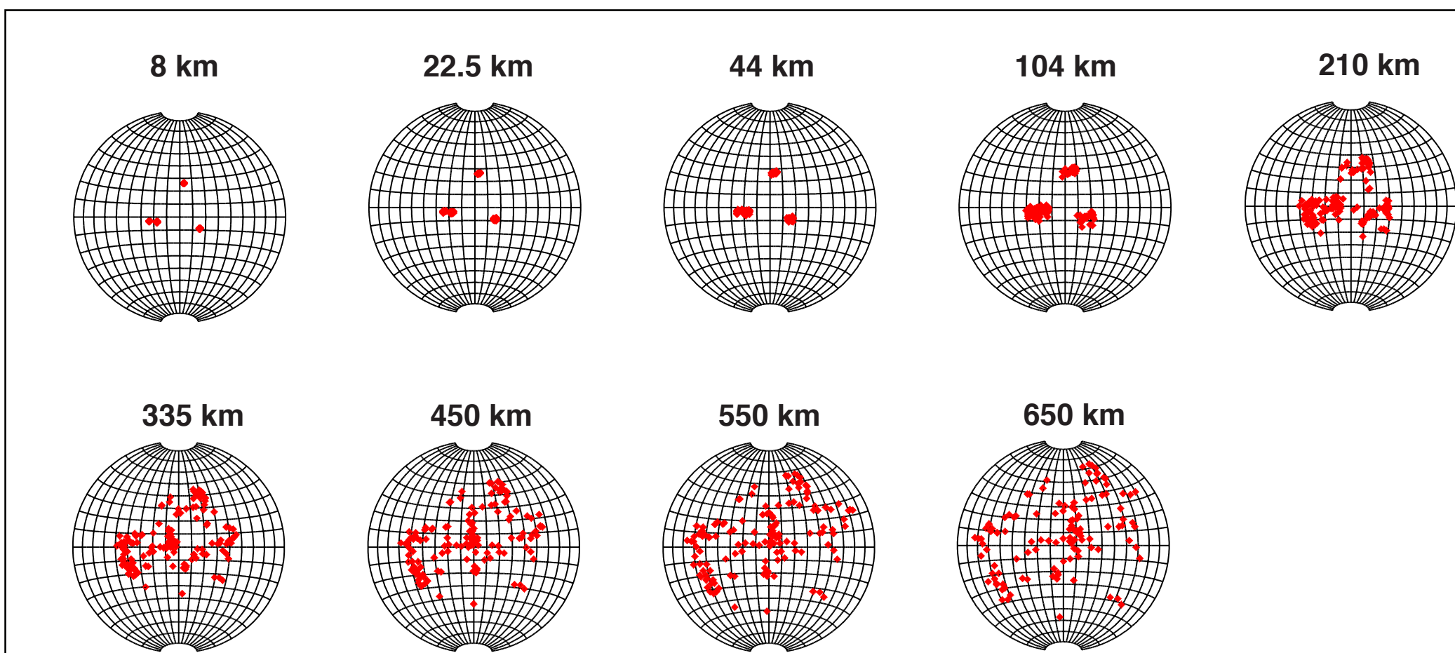
Figure 3: Pierce-points (red dots) for P-wave rays at each of the modeled layer boundaries. Shallow ray coverage is sparse, but increases with depth.
