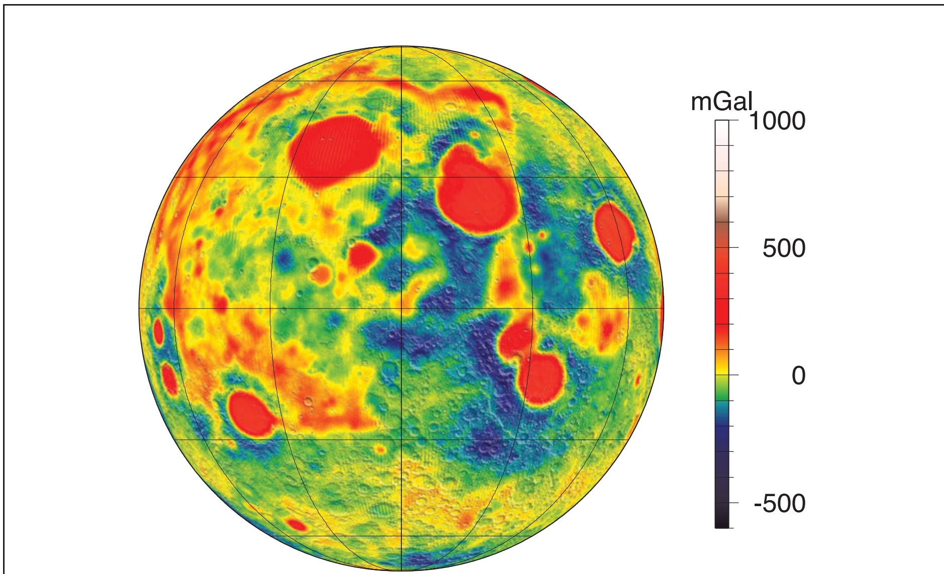
Figure 5: Near-side centered Bouguer gravity anomaly.
