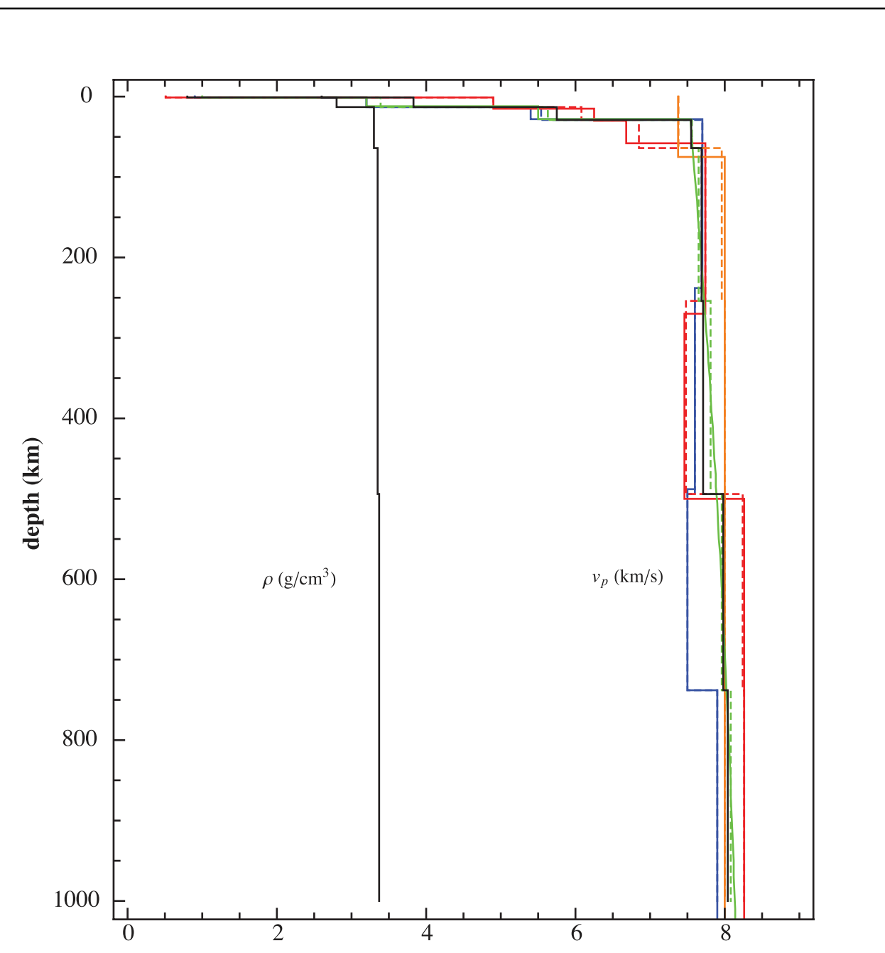
Figure 4: Average velocity (and density) model (black lines) compiled from four popular lunar structure models: red [3], blue [4], orange [5], green [6].
