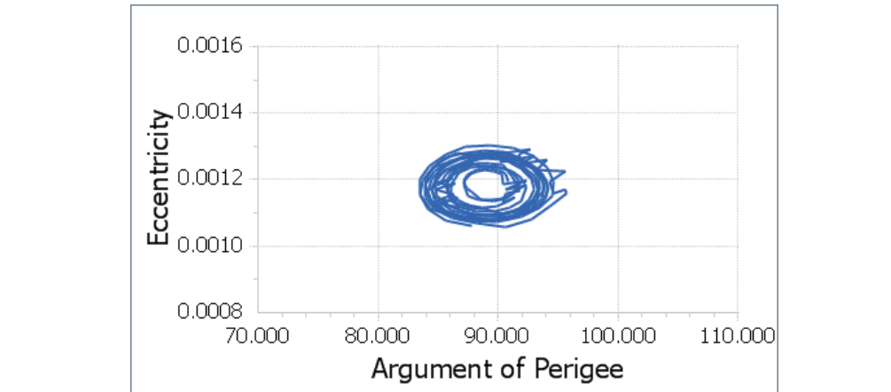
Figure 12. Frozen orbit (eccentricity, argument of perigee) for all no-slew mirror pole maneuvers over four years. The mirror pole strategy shows much larger deviations than the others, but still within operational constraints
