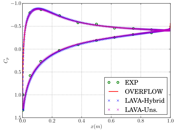
Figure 21. Pressure coefficient distribution on surface of NACA 0012 airfoil. Experimental data, hybrid and unstructured approaches of LAVA results are shown.
