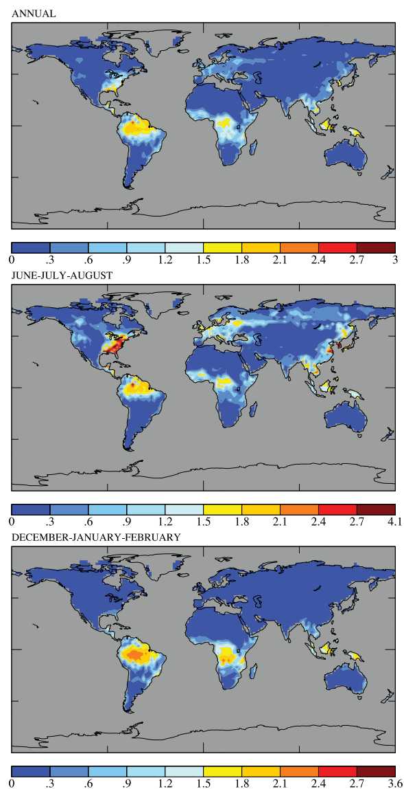
Fig. 1b. Spatial distribution of annual and seasonal average modeled isoprene emission in \text{mgC m}^{-2} \text{h}^{-1} in the control run SimCONT.
