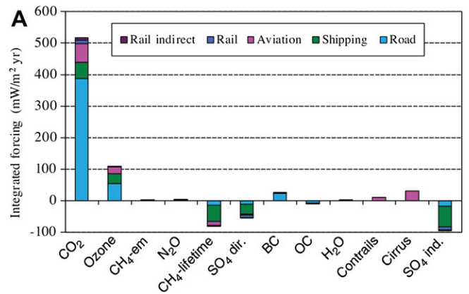
Fig. 38. Integrated radiative forcing of current emissions, by substance and transport subsector, over different time horizons. (A) Integrated global mean RF(mW m 2 yr) due to 2000 transport emissions, time horizon H = 100 years. (From Fuglestedt et al., 2008)
