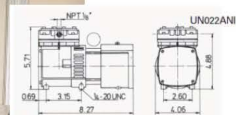
Recycle Pump
