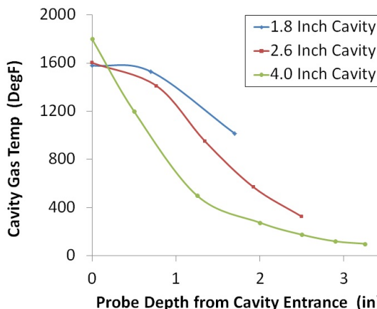
Figure 5. Example Cavity Gas Temperatures.
