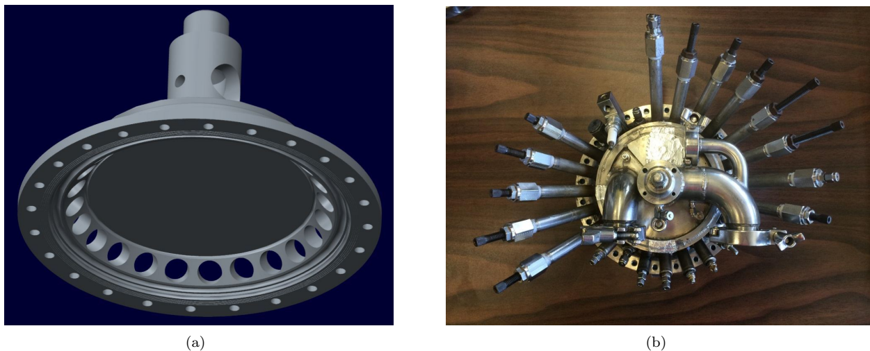
Figure 4. Morpheus main engine injector acoustic cavity layout. (a) Acoustic cavity ring at 45 deg to faceplate. (b) Tunable acoustic cavity configuration.
