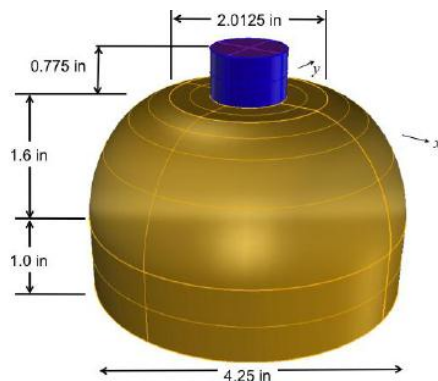
Figure 8: Final Ground Plane Geometry
