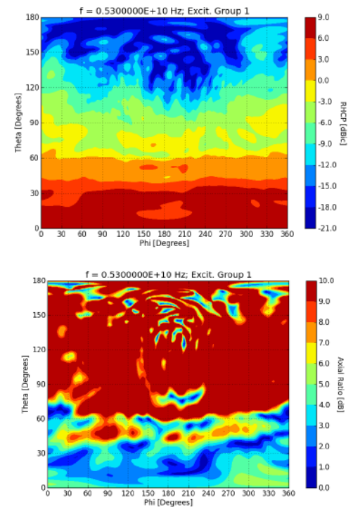
Figure 9: Ground Plane Design RF Coverage
