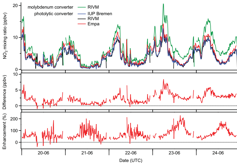
Fig. 13. Top panel: comparison of four in-situ atmospheric NO 2 sampling instruments. The green line represents the instrument with a conventional hot-plate molybdenum converter, whereas the black, red and blue lines represent the instruments with a photolytic converter, from RIVM, Empa, and IUP Bremen, respectively. The middle and lower panels show the absolute and relative difference (enhancement) between the mixing ratio derived from the instrument with molybdenum converter and the average mixing ratio derived from the three other instruments.
