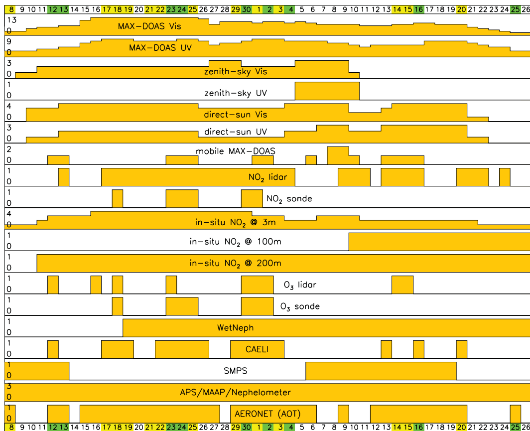
Fig. 9. Number of instruments which have collected data on each day during the CINDI campaign and for each of the instrument types. The day numbers in June and July are at the top and bottom of the figure. The yellow and green days are days of category A and B, respectively (see Sect. 3.1).
