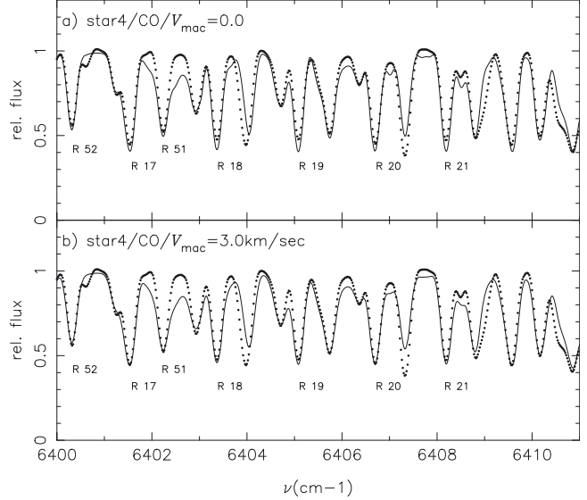
Fig. 10. T analysis: a) observed spectrum (dots, relative flux vs. wave number) and model spectrum (solid line) with a macroturbulence of zero, for the CO lines between 1.5601 and 1.5625 \mu\text{m} of Star 4 ; b) the same as a) but with a macroturbulence of 3.0 \text{ km s}^{-1} .
