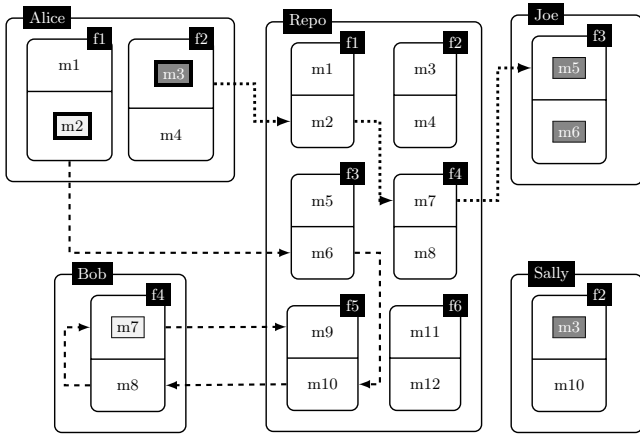
Figure 1: Change Scenarios
