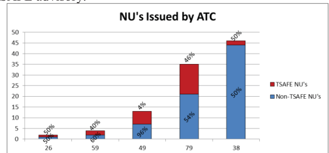
Figure 16. Total NU's issued by a controller in the presence and absence of TSAFE advisories.
