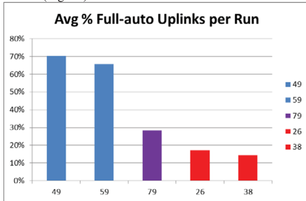
Figure 14. Average percentage of uplinks in a run that were full-auto, i.e. the green bars from Fig. 13.
