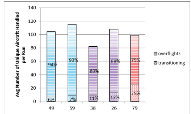
Figure 8. Number of aircraft handled on average by a sector controller in a single run.
