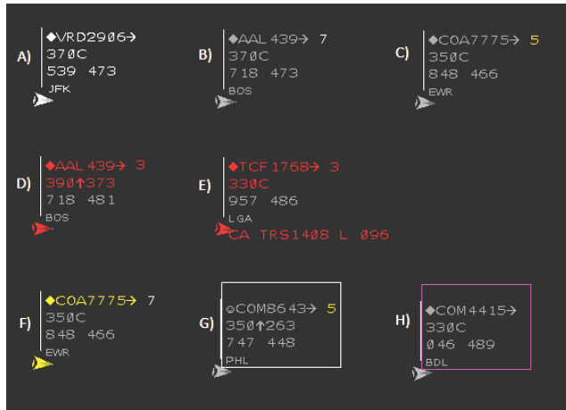
Figure 3. Expanded data tag examples.
