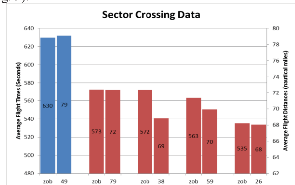
Figure 9. Average aircraft sector crossing times (secs) and distances (nm).
