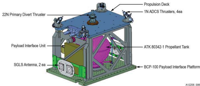
Figure 2: Conceptual Design of AF-M315E Propulsion System [1] ADCS: Attitude Determination and Control SGLS: Space to Ground Link System
