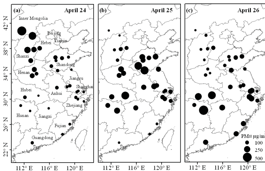
Fig. 4. Regional distribution of PM 10 concentration ( \mu\text{g m}^{-3} ) during 24–26 April (Data source: Ministry of Environment Protection of the PRC, http://www.zhb.gov.cn/ ).
