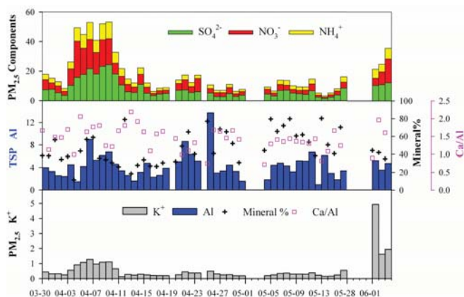
Fig. 6. Time series of (a) SO_4^{2-} , NO_3^- , and NH_4^+ concentration ( \mu\text{g m}^{-3} ) in PM_{2.5} (b) Al concentration ( \mu\text{g m}^{-3} ), the fraction of mineral aerosol, and the elemental ratio of Ca/Al in the total suspended particles (TSP) (c) K^+ in PM_{2.5} , during the whole study period (Missing data were due to rainfall or malfunction of instruments).
