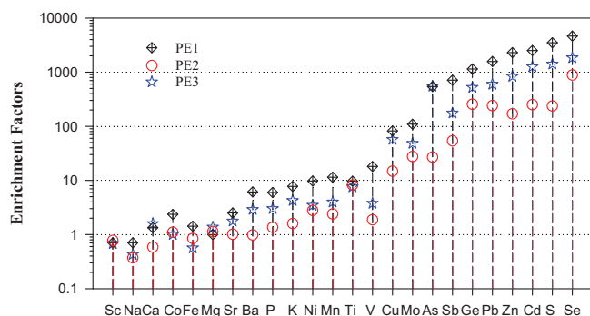
Fig. 7. The average enrichment factors (EF) of various elements during PE1, PE2, and PE3, respectively.
