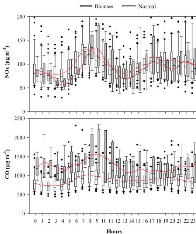
Fig. 11. The diurnal variation of CO and NO x concentrations ( \mu\text{g m}^{-3} ) during the biomass burning period (gray box) and normal period (white box), respectively. Diurnal mean values are connected by the red spline curves; bottom and top of the boxes represent the 25 and 75 % limits, respectively; and bottom and top short lines represent the minimum and maximum values, respectively. Black dots represent the outliers.
