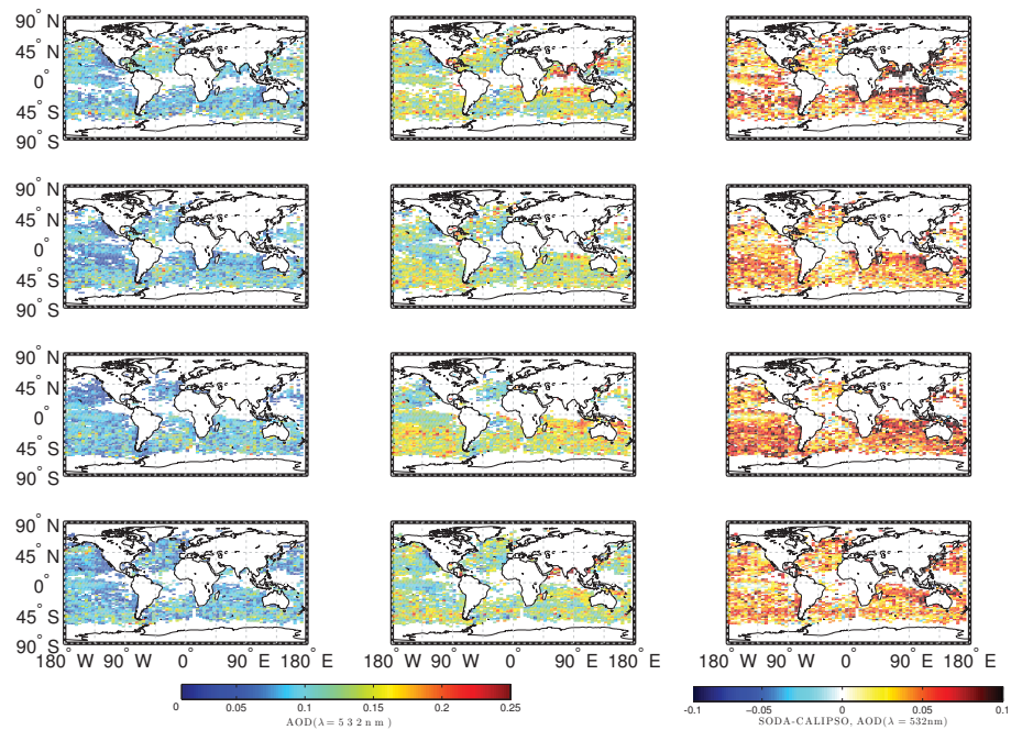
Fig. 1. Seasonal median AOD values from CALIOP and SODA (columns 1 and 2) and the difference (SODA – CALIOP) plot (column 3) for December–February (row 1), March–May (row 2), June–August (row 3), September–November (row 4) plotted on a 2^\circ \times 5^\circ latitude longitude grid. “No Data” is shaded white and is defined as grid cells failing quality control algorithm (see text for details).
