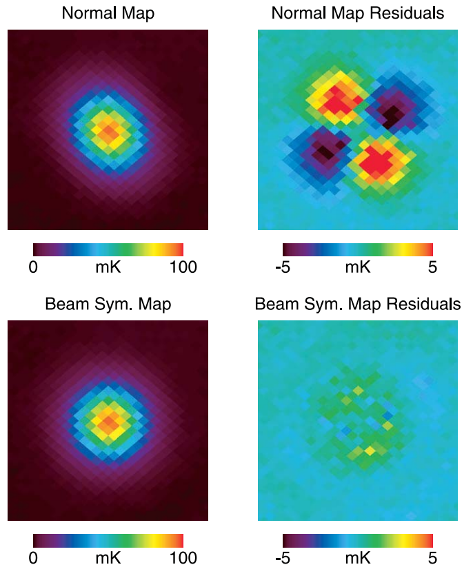
Figure 7. K -band images of supernova remnant Tau A (3C 144), at [J2000.0] position ( 05^{\text{h}}34^{\text{m}}31^{\text{s}}, 22^{\circ}01' ) from the first year of WMAP observations. The left panels display the total intensity and right the residuals after removal of a best-fit circularly symmetric beam profile. The maps generated with the new partial deconvolution processing (bottom) display significantly reduced beam asymmetry compared with those generated with the standard processing (top). In other words, the apparent asymmetry in Tau A seen in the top left is a result of the asymmetric K -band beam and is not intrinsic to Tau A. The degree of a source's apparent asymmetry is dependent on its sky position and the WMAP frequency at which it is observed: the effect is most pronounced for bright K -band sources at low ecliptic latitudes (Section 4.2). As such, we display the K -band observations of Tau A to demonstrate the effectiveness of the deconvolution in a worst case of beam asymmetry in the normally processed maps.
