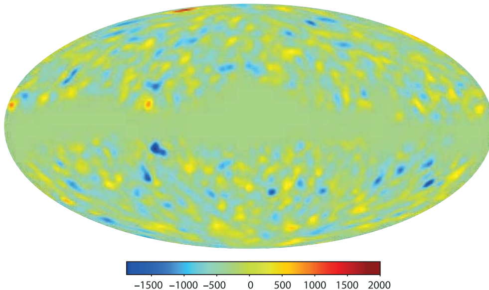
Figure 41. Visual test for sky location dependent systematics: skymap showing the contribution of different parts of the sky to the f_{\text{NL}}^{\text{orth}} estimator, in units of ‘‘ f_{\text{NL}}^{\text{orth}} per steradian.’’ We do not detect any significant localized features in this map.
