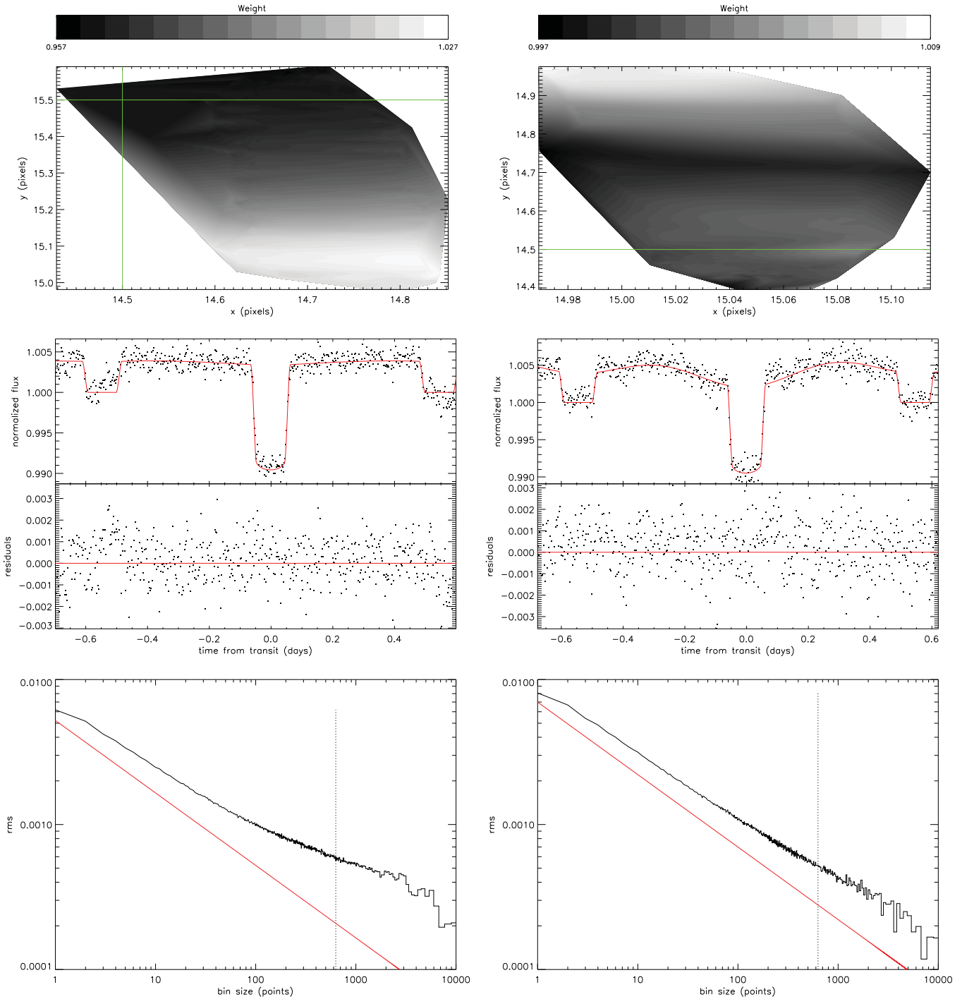
Figure 3. WASP-12b at 3.6 \mu\text{m} (left) and 4.5 \mu\text{m} (right), where we have corrected for IPSVs using the Ballard et al. (2010) point-by-point decorrelation, as described in Section 3.2.1. The upper panels show the IPSV map determined from our science data, with pixel edges shown in green. The second panels show the corrected data with best-fit astrophysical model and residuals. The bottom panels show the scatter in the residuals as a function of binning; the red line shows the photon noise limit; the vertical dotted line denotes the timescale of ingress/egress.
