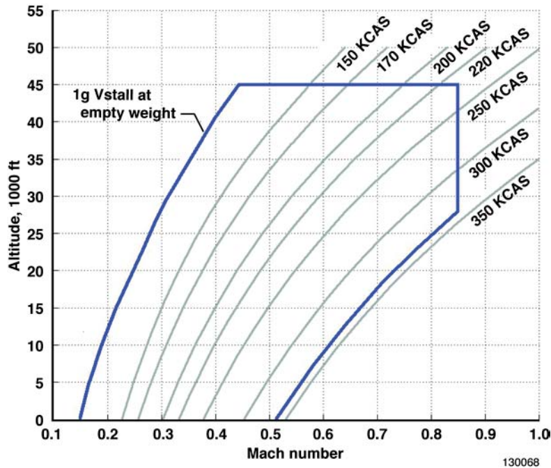
Figure 3. SCRAT flight envelope.
