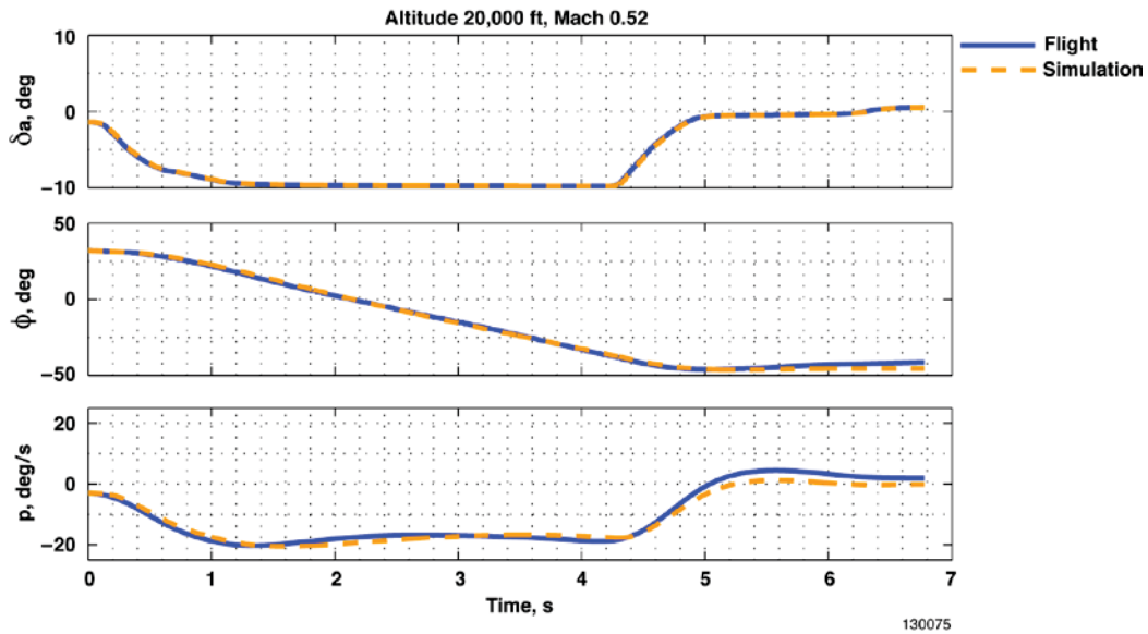
Figure 17. Sample comparison between simulation and flight data.
