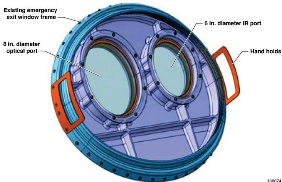
Figure 15. Modified emergency exit window.
