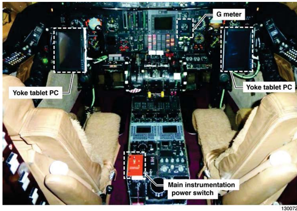
Figure 10. SCRAT cockpit.
