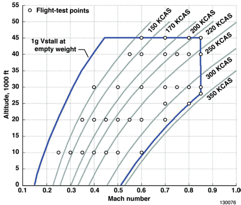
Figure 21. Baseline characterization flight data points.
