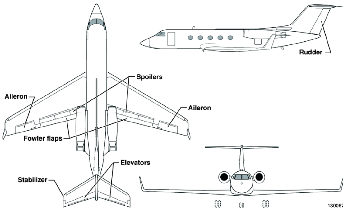
Figure 2. 3-view of the SCRAT.
