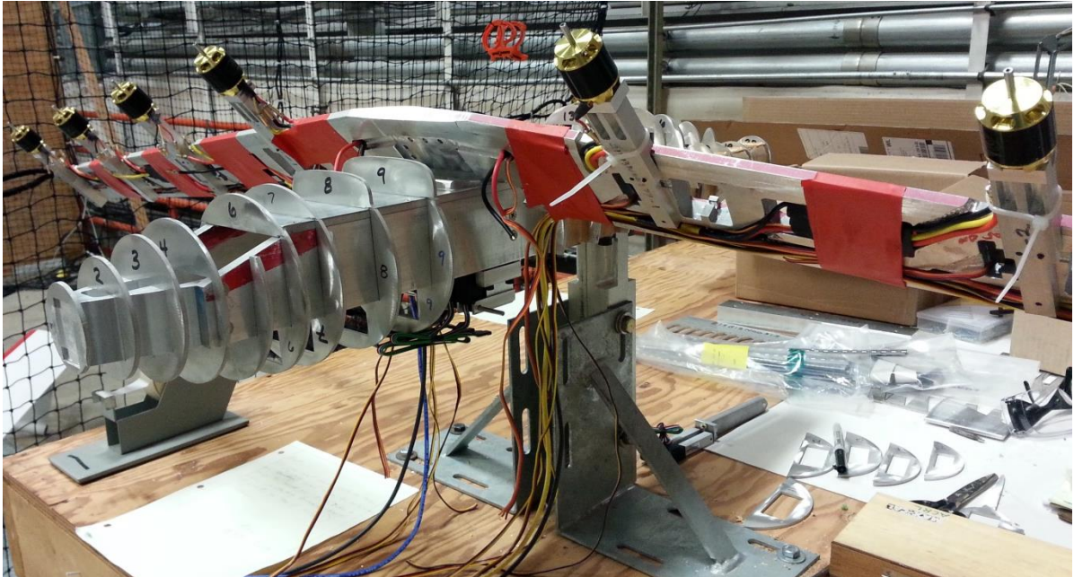
Figure 6. GL-10 Wind Tunnel Model Wing Motor Wiring
