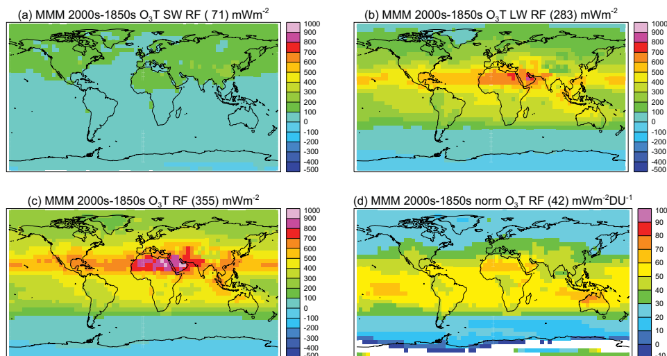
Fig. 3. Multi-model mean, annual mean tropospheric ozone radiative forcings ( \text{mW m}^{-2} ), for: (a) SW; (b) LW; (c) total (SW+LW); and (d) total RF normalised by tropospheric column ozone change (Fig. 1f) ( \text{mW m}^{-2} \text{DU}^{-1} ). The normalised RF is masked (white boxes) where the change in ozone column is less than 0.25 DU. Area-weighted global mean values are given in brackets. Figure S2 shows equivalent plots for all individual models.
