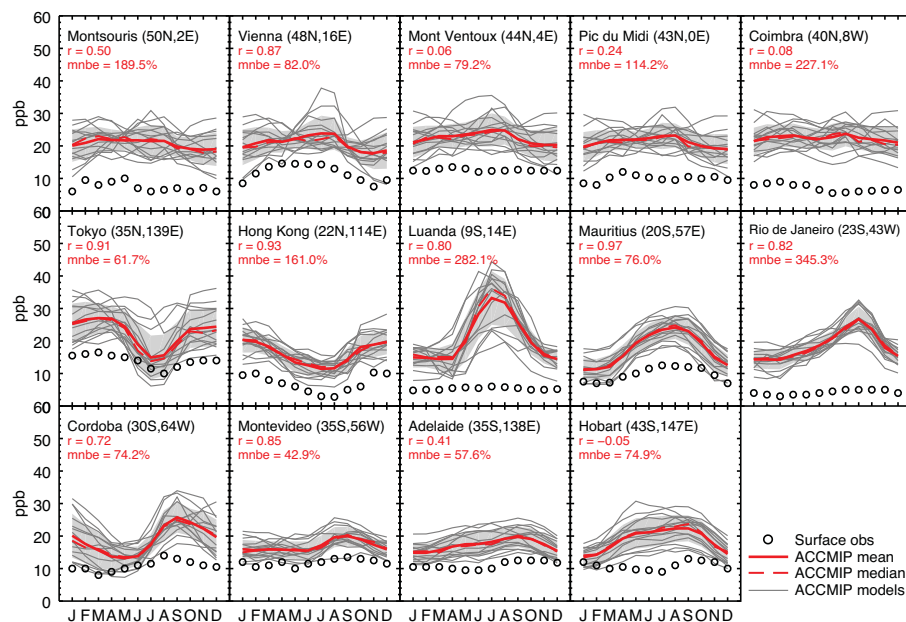
Fig. 2. Comparison of 1850s modelled seasonal cycles of ozone (lines) with observations of ozone (circles) at 14 surface sites. The observations have large, but unquantified uncertainties, so no error bars are included. The correlation ( r ) and the mean normalised bias error (mnbe) of the mean model to the observations are also shown for each site.
