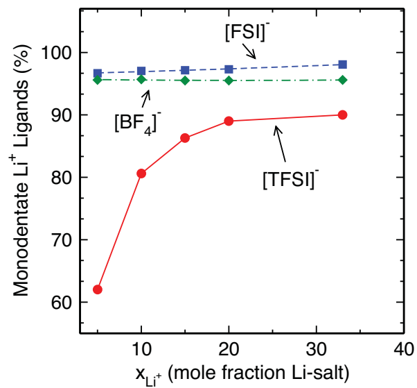
Figure 5: Proportion of Li^+ ligand anions having monodentate bonds as a function of Li-salt doping at T = 298 K.
