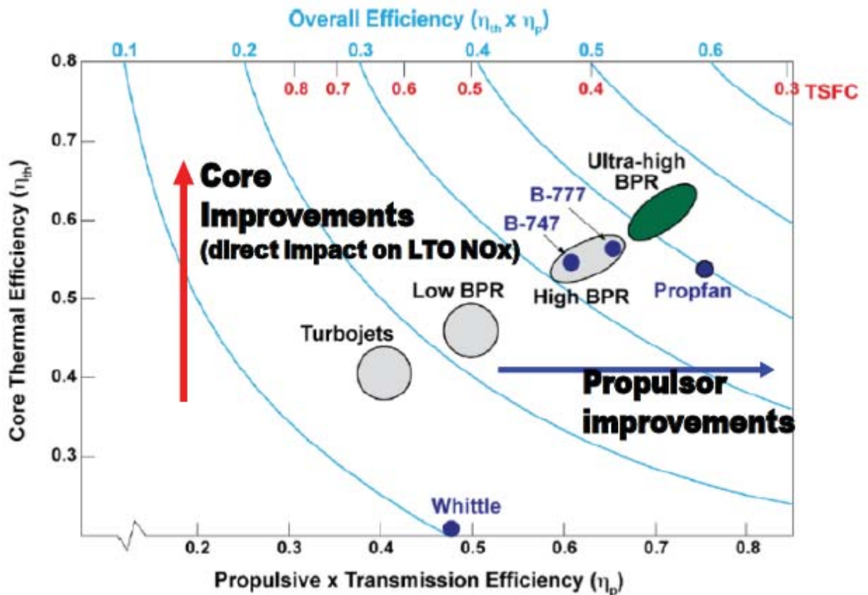
Figure 16: Trends in overall propulsion efficiency and thrust specific fuel consumption with core and propulsor improvements. Future improvements require increases in both thermal and propulsive efficiency.
