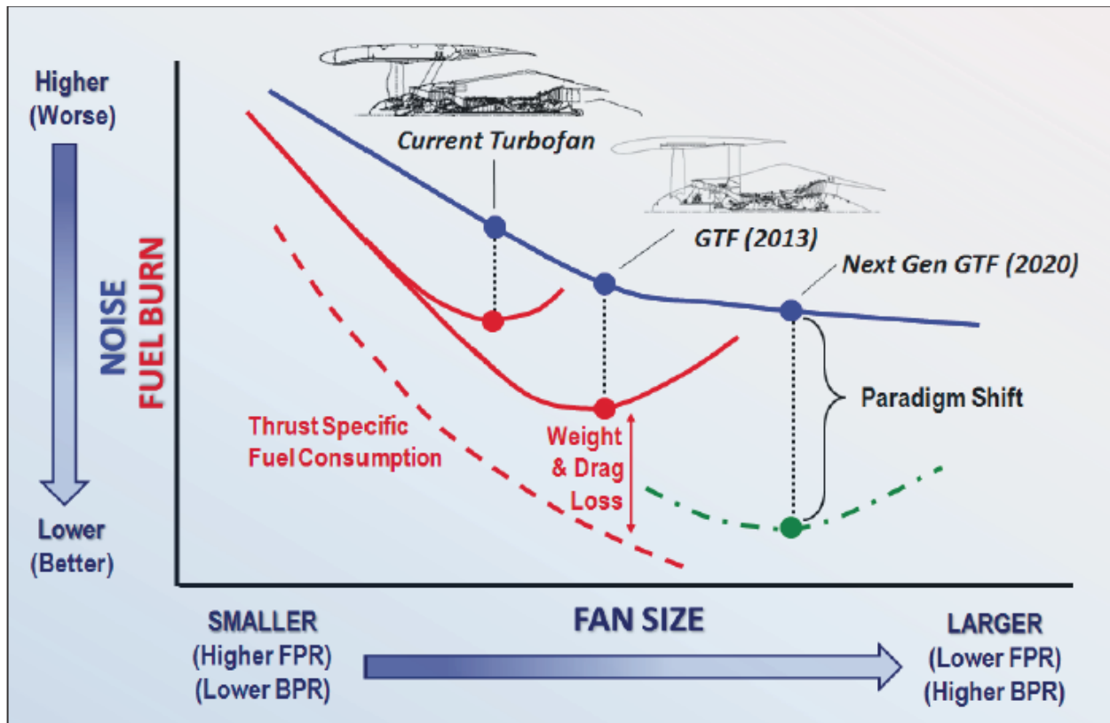
Figure 11: Effect of fan size, bypass ratio, and fan pressure ratio on fuel burn.
