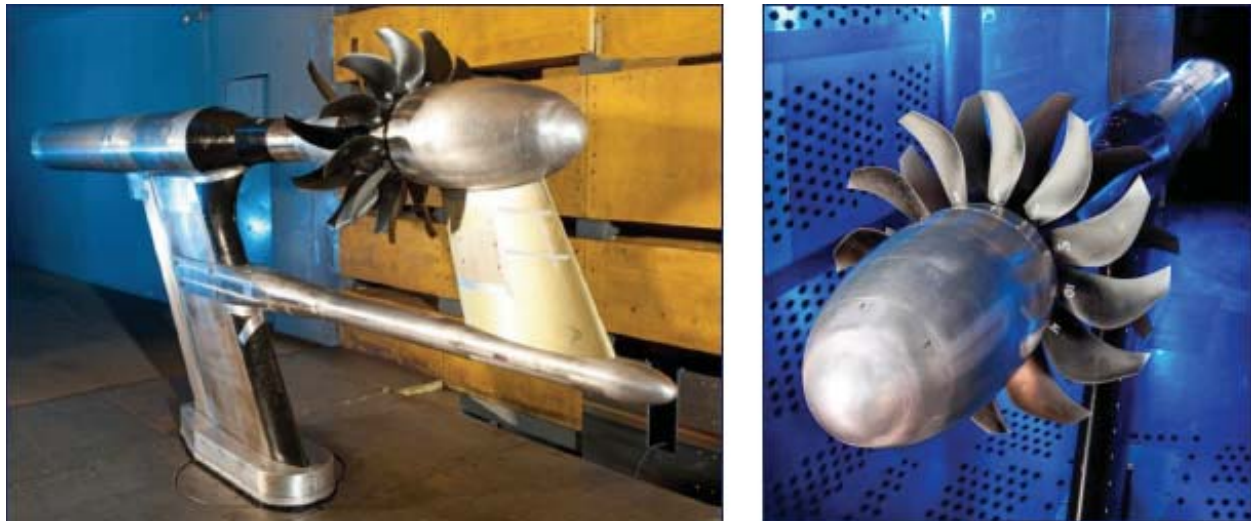
Figure 8: The Open Rotor Propulsion Rig installed in the 9x15 Low Speed wind tunnel on the left and on the right it is installed in the 8x6 Transonic Wind Tunnel in preparation for performance testing at cruise Mach of ~0.8.
