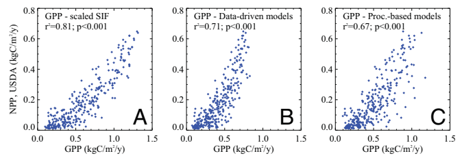
Fig. 5. Comparison of net primary production (NPP) estimates over the US Corn Belt (35°N–50°N, 80°W–105°W) from the USDA agricultural inventory (8) with crop GPP estimates from SIF retrievals (A) and data-driven and process-based model ensembles (B and C). Points correspond to 1° grid boxes with fraction of cropland area higher than 20%. GPP and NPP values are given in per-total-area units (see SI Appendix, NPP Data from Agricultural Inventories ). The squared Pearson's correlation coefficient r^2 and the P value of the comparisons are shown. An analogous comparison with the inventory-based NPP from Monfreda et al. (7), which also includes Western Europe, can be found in SI Appendix, NPP Data from Agricultural Inventories .
