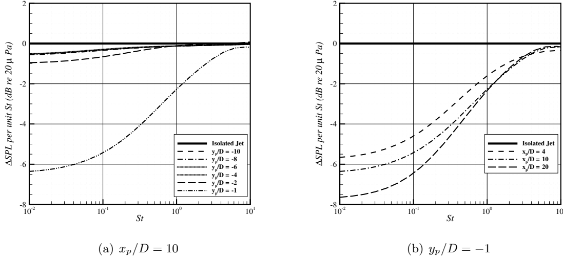
Figure 19. Predicted attenuation using the model of Tam and Auriault [19] for the free and installed jet at R/D = 100 and \Psi = 90 deg. The jet operates at M_j = 1.29 and TTR = 1.00 from the convergent SMC016 nozzle with D = 0.0508 m. Part a) shows plate locations at y_p/D = -1, -2, -4, -6, -8, and -10 laterally from the jet centerline and x_p/D = 10 . Part b) shows the plate located at y_p/D = -1 and x_p/D = 4, 10, and 20 .
