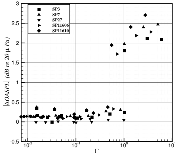
Figure 21. \Delta\text{OASPL} , relative to the free jet, for each condition shown in Tables 1 and 2.
