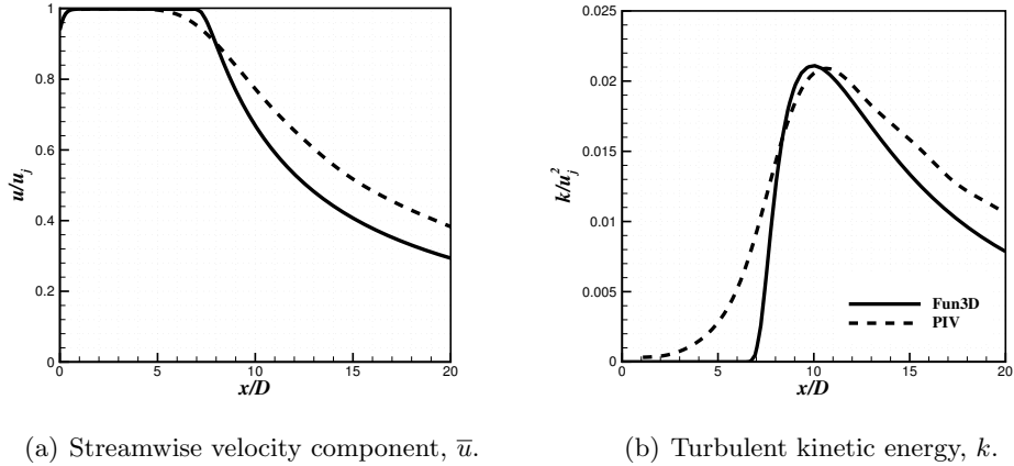
Figure 13. The steady RANS a) \bar{u} and b) k along the jet centerline compared with the measurement of Bridges and Wernet [52]. The jet operates at M_j = 0.513 and TTR = 1.00 from the convergent SMC000 nozzle.
