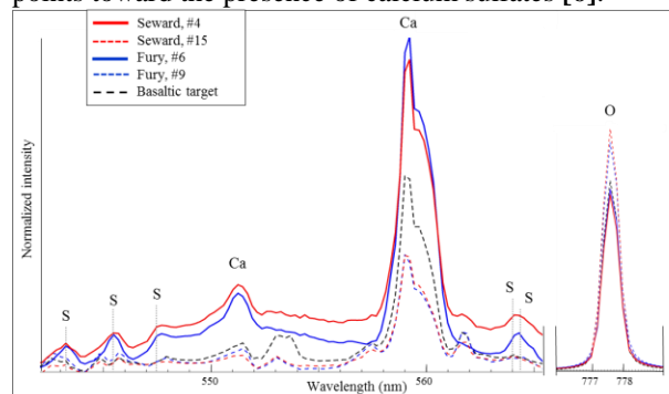
Figure 1 : Example of LIBS/ChemCam targets displaying Ca-sulfate signature (solid spectra), and surrounding points of the same target (dotted spectra) without Ca-sulfate signature. The ChemCam calibration target in black spectra is shown for comparison with a classical silicate rock.
