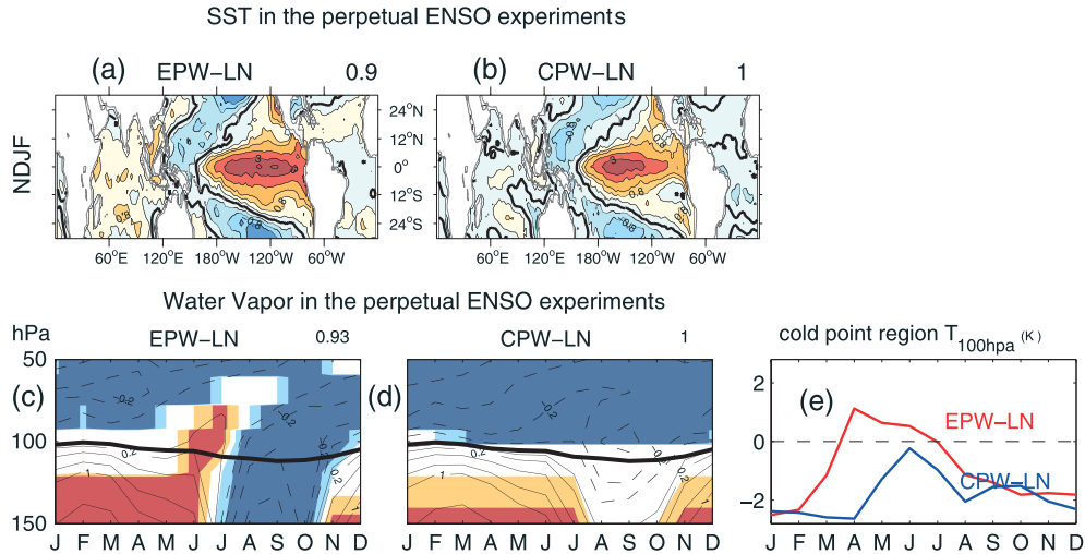
Figure 1. Sea surface temperature, tropical water vapor ( 20^{\circ}\text{S} – 20^{\circ}\text{N} ), and cold point temperature anomalies in the perpetual CPW and EPW GEOSCCM integrations. (a, b) Contours are shown at \pm 0.4 , \pm 0.8 , \pm 1.2 , \pm 2 , and \pm 3 ; region with large warming (cooling) are colored red (blue). (c–d) Contours are shown at \pm 0.1 , \pm 0.2 , \pm 0.4 , \pm 0.7 , \pm 1 ppmv, and regions with anomalies significant at the 90% (99%) level are colored orange (red) or light blue (dark blue). A solid black contour indicates the climatological position of the tropopause. The pattern correlation between the CPW and EPW anomalies are shown in the title of Figure 1a–1d. (e) The temperature anomaly associated with EN averaged in the cold point regions at 100 hPa (as defined in section 2) for each calendar month.
