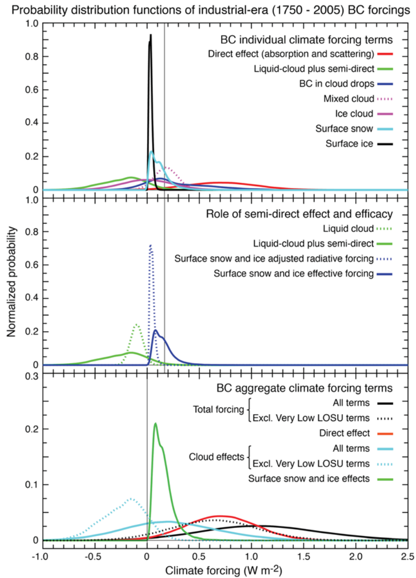
Figure 36. Probability distribution functions (PDFs) of industrial-era (1750–2005) forcings for BC climate forcing terms. Top: Individual PDFs for each climate forcing term. Middle: Before and after PDFs showing the role of the semi-direct effect in modifying the liquid cloud climate forcing term and the role of efficacy in modifying the BC-in-snow and BC-in-ice combined forcing term. Bottom: PDFs of the aggregated climate forcing components and the total climate forcing (see text for details). In the bottom panel, aggregated forcings are presented in two ways: with very low LOSU terms included (solid lines) or excluded (dotted lines). Probabilities are normalized to unity for all terms. Note the different vertical scale in the bottom panel.
