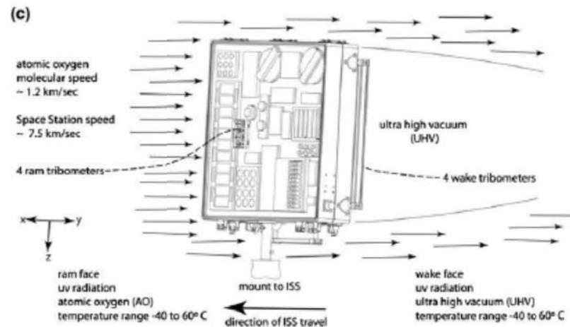
Eight POD units in MISSE Rack
