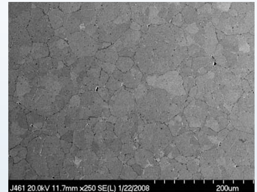
60NiTi microstructure
