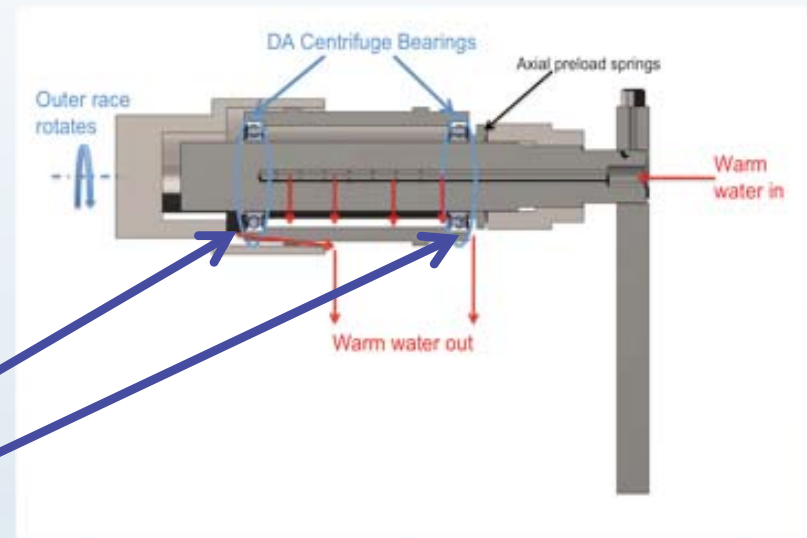
DA Centrifuge Bearing Test Rig Spindle Components
