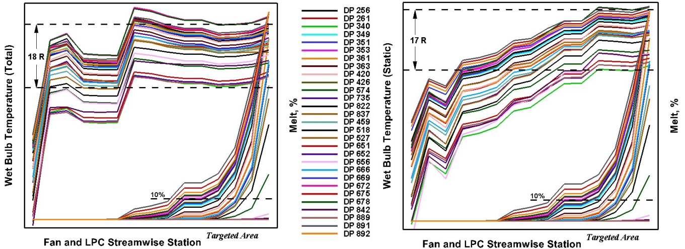
a) Figure 9: Flow analysis of the fan-core and LPC stage at the test data points which resulted in no engine icing events. The calculated wet bulb temperature based on the total temperature is shown in (a) and the static temperatures are illustrated in (b).
