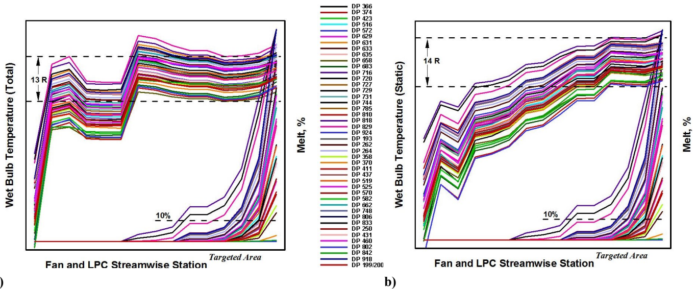
a) Figure 8: Flow analysis of the fan-core and LPC stage at the test data points which resulted in gradual (slow) engine icing events. The calculated wet bulb temperature based on the total temperature is shown in (a) and the static temperatures are illustrated in (b).
