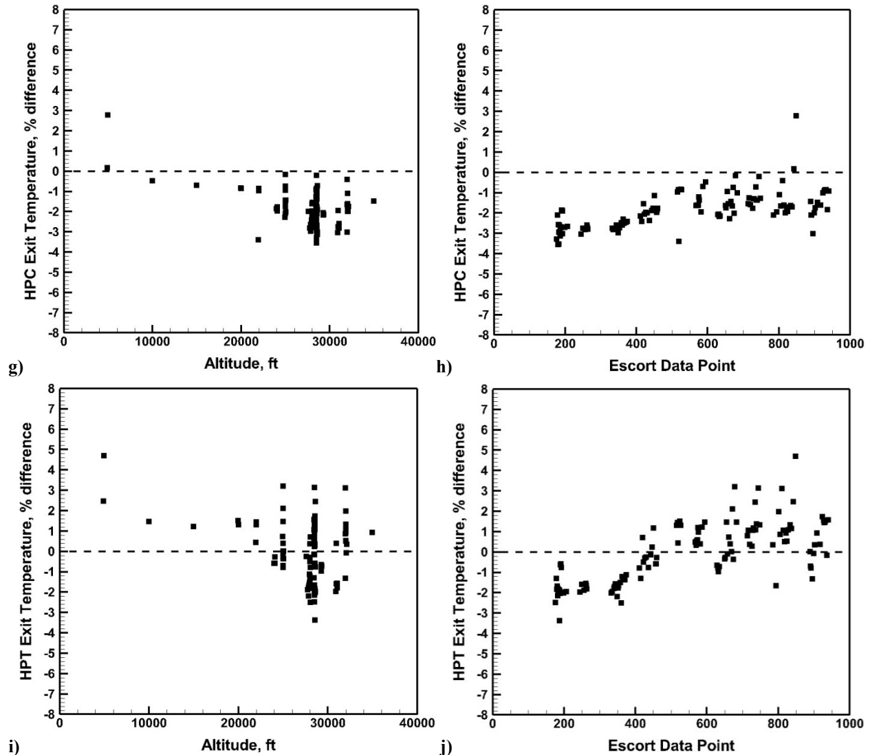
Figure 12: The percent difference between the measured data in the PSL and the values calculated with the CD engine system model (air flow, fuel flow, HPC exit pressure, HPC exit temperature, and HPT exit temperature) are shown vs. altitude (a, c, e, g, i) and vs. Escort data point number (b, d, f, h, j).
