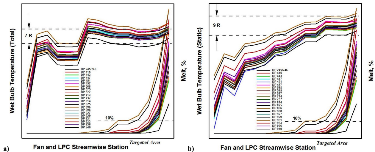
Figure 7: Flow analysis of the fan-core and LPC stage at the test data points which resulted in an imminent (fast) engine icing event. The calculated wet bulb temperature based on the total temperature is shown in (a) and the static temperatures are illustrated in (b).
