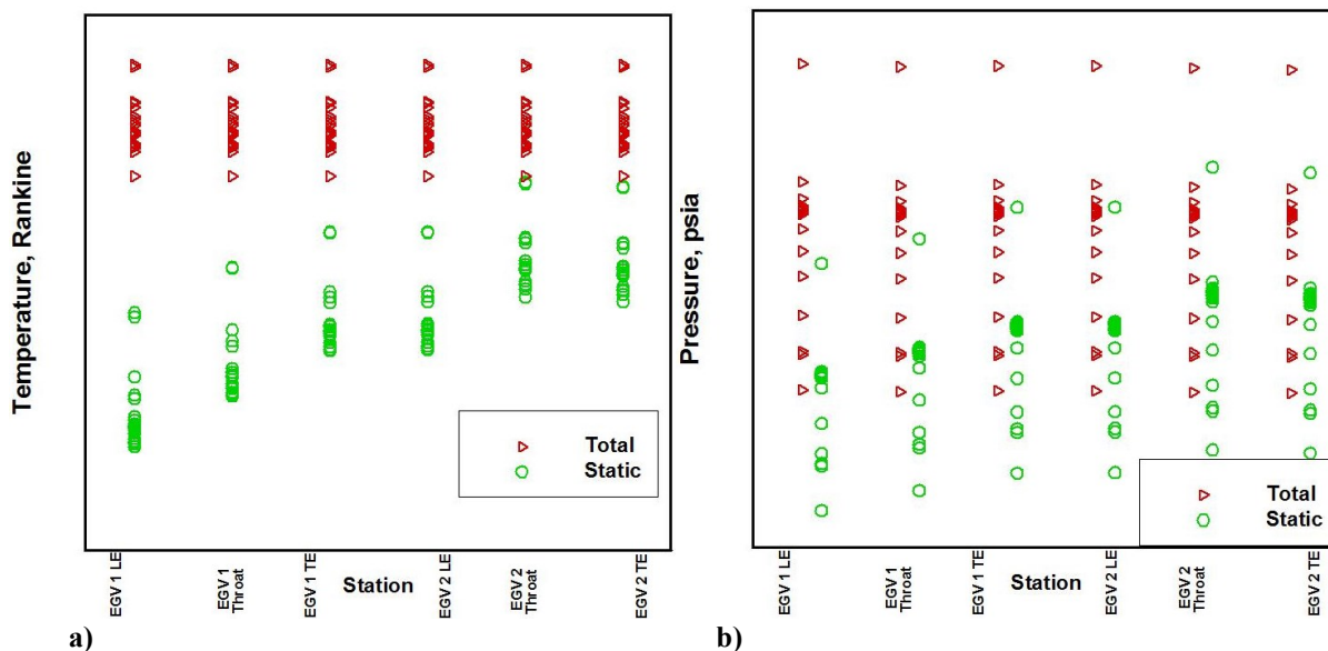
Figure 11. The air temperatures (a) and pressures (b) at the EGV tandem stator 1 and 2 leading and trailing edges, as calculated by the computer model, for engine data points that experienced imminent (fast) ice accretion rates.
