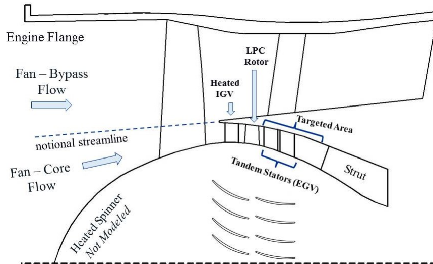
Figure 6: Schematic of the fan and low pressure compressor portion of the engine tested in the PSL with ice crystal ingestion, illustration the tandem stators of the EGV, and the Targeted Area.
