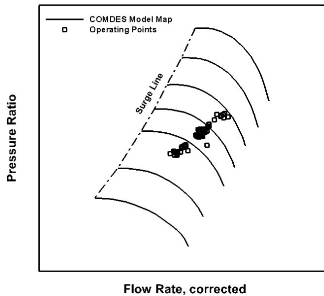
Figure 10: The PSL test data operating points superimposed onto the fan-core and LPC characteristic performance map. These points represent all the PSL data points that are shown in Figures 7, 8, and 9.
