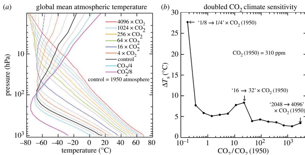
Figure 7. (a) The calculated global mean temperature for successive doublings of \text{CO}_2 (legend identifies every other case) and (b) the resulting climate sensitivity ( 1 \times \text{CO}_2 = 310 \text{ ppm} ).
