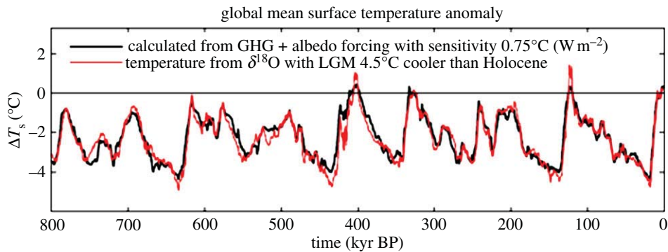
Figure 6. Calculated surface temperature for forcings of figure 5c with a climate sensitivity of 0.75°C per W m -2 , compared with 2 \times \Delta T_{\text{do}} . Zero point is the Holocene (10 kyr) mean.
