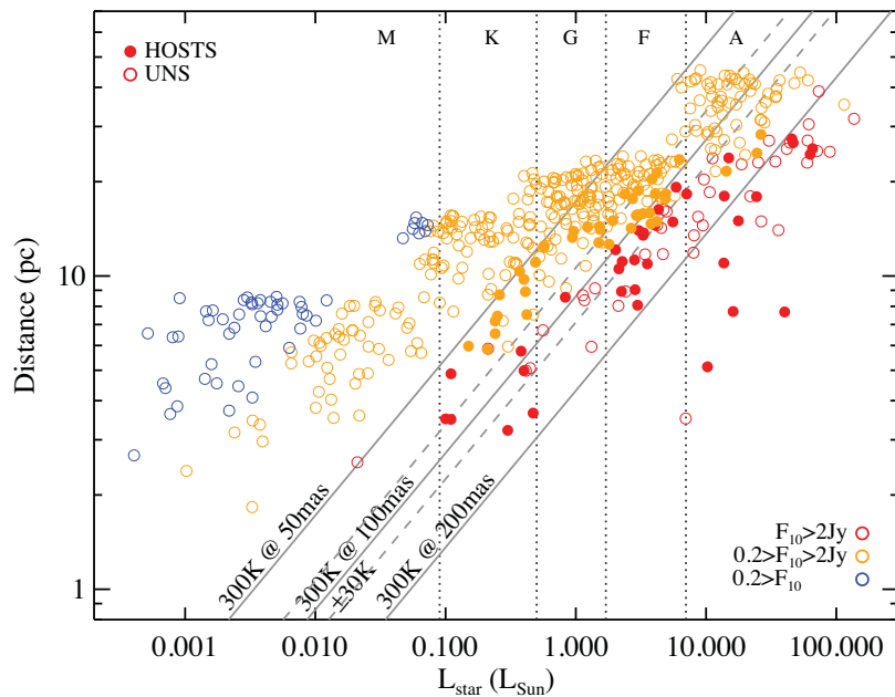
Figure 5. The distance of stars from Sun sample as a function of luminosity, grouped according to 10- \mu m flux. The open circles represent the UNS sample, and the red and orange closed circles represent the HOSTS sample. The solid lines denote distance as a function of luminosity given a blackbody at a temperature of 300K at angular scales of 50, 100, and 200 mas, and the dashed lines \pm 30K from the 300K line. Dotted lines are approximate boundaries in luminosity for the spectral classes (Weinberger et al. [24]).
