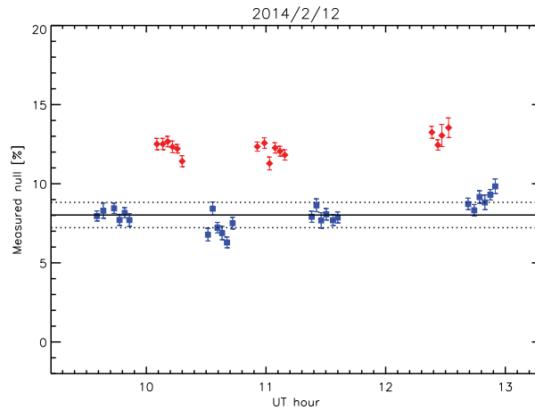
Figure 9. Null measurements for \eta Crv in which only the best 5% of the measurements are averaged. The red symbols denote the measurements of \eta Crv and the blue symbols are measurements of the calibrator stars. The black line is an average of the calibrator measurements, and the average error in the null measurements for the calibrators is indicated by the dotted lines. The excess is detected in the N' band ( 9.81\text{--}12.41\ \mu\text{m} ) over a field-of-view of \sim 140 mas in radius, corresponding to \sim 2.6 AU at the distance of \eta Crv.
