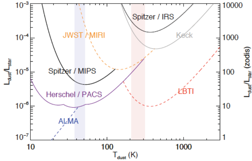
Figure 3. Comparison of the sensitivity of major instruments as a function of dust temperature, using L_{\text{dust}}/L_{\text{star}} as a measure of sensitivity, where L_{\text{dust}} is the luminosity of dust and L_{\text{star}} is the luminosity of a star. Note that LBTI has the best sensitivity of all existing and near-term instruments for dust between 150 and 1000 K, including the MIRI instrument on JWST. (Adapted from Roberge et al. [4]).
