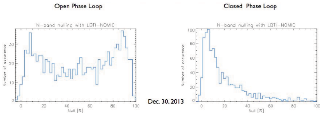
Figure 7. Results obtained in December 2013 when the PhaseCam loop was closed for the first time. The panel displays a histogram of a sequence of null measurements before the phasing loop was closed. In this plot, note that the number of measurements of the null depth range from near zero to 100%, which is a consequence of the random variation of the path length, and hence phase, between the two telescopes. The right panel is the histogram of the nulling sequence with the phase loop closed. In this plot the histogram clearly shows most of the measurements peaking close to a null depth of a few percent, consistent with the residual rms phase variation.
