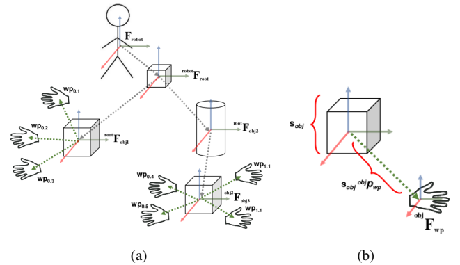
Fig. 4. Diagram (a) shows the generic structure of ATs. Diagram (b) shows the template scaling methodology.
