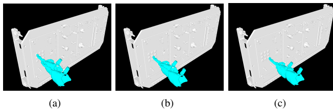
Fig. 10. Three different stored trajectories for pushing (different) buttons on the ISS Taskboard.
