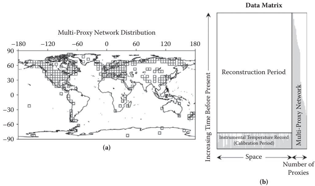
FIGURE 4.4 (a) Representation of the global distribution of the most up-to-date global multi-proxy network used by Mann et al. [58]. Grey squares indicate the 5° grid cells that contain at least one proxy in the unscreened network from ref. [58]. (b) Schematic of the data matrix for temperature field reconstructions spanning all or part of the CE. Grey regions in the data matrix are schematic representations of data availability in the instrumental temperature field and the multi-proxy matrix. White regions indicate missing data in the various sections of the data matrix.
