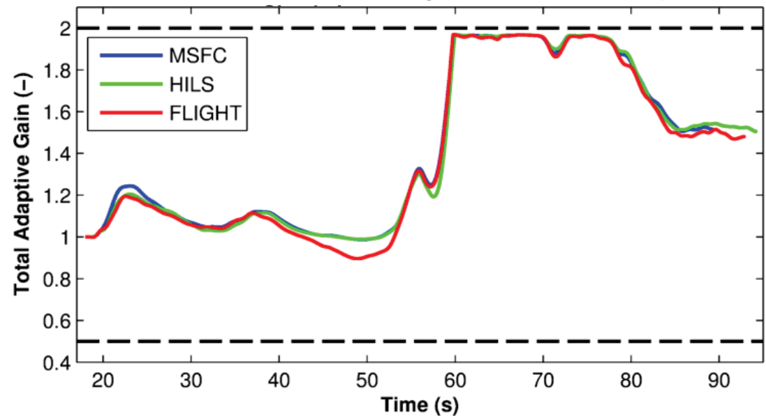
HILS – Armstrong’s Hardware-In-the-Loop
