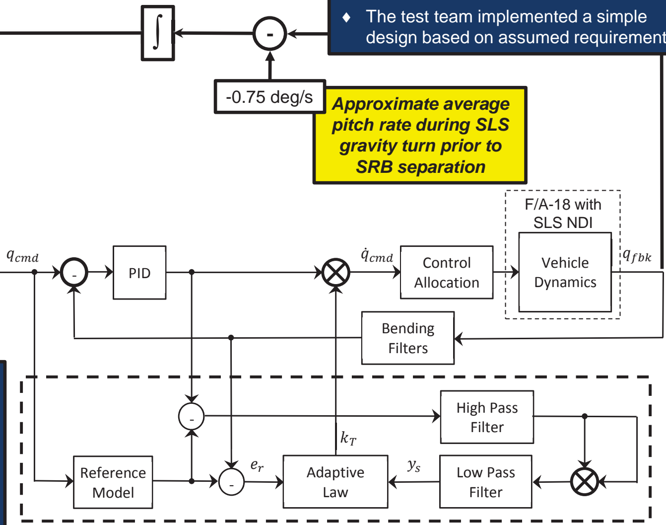
Adaptive Augmenting Control Algorithm
