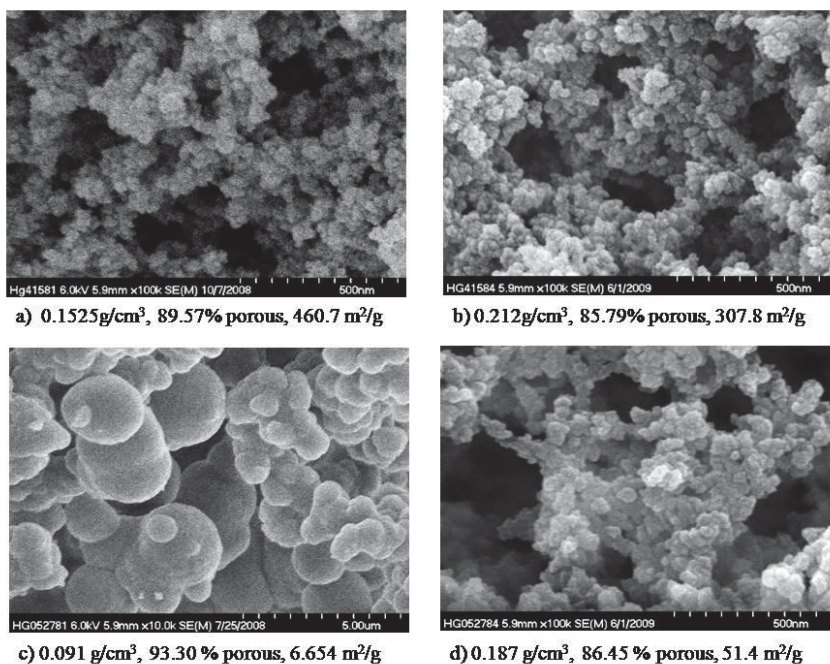
Figure 11. SEM images of a) sample 4 (0.2 mol/l BTSPD) and b) sample 7 (0.3 mol/l BTSPD) made using 0.5 mol/l TMOS, compared to samples made with 0.1 mol/l TMOS c) sample 20 (0.2 mol/l BTSPD) and d) sample 23 (0.3 mol/l BTSPD). (Reproduced from Publication 24 with the permission from The Royal Society of Chemistry.)
