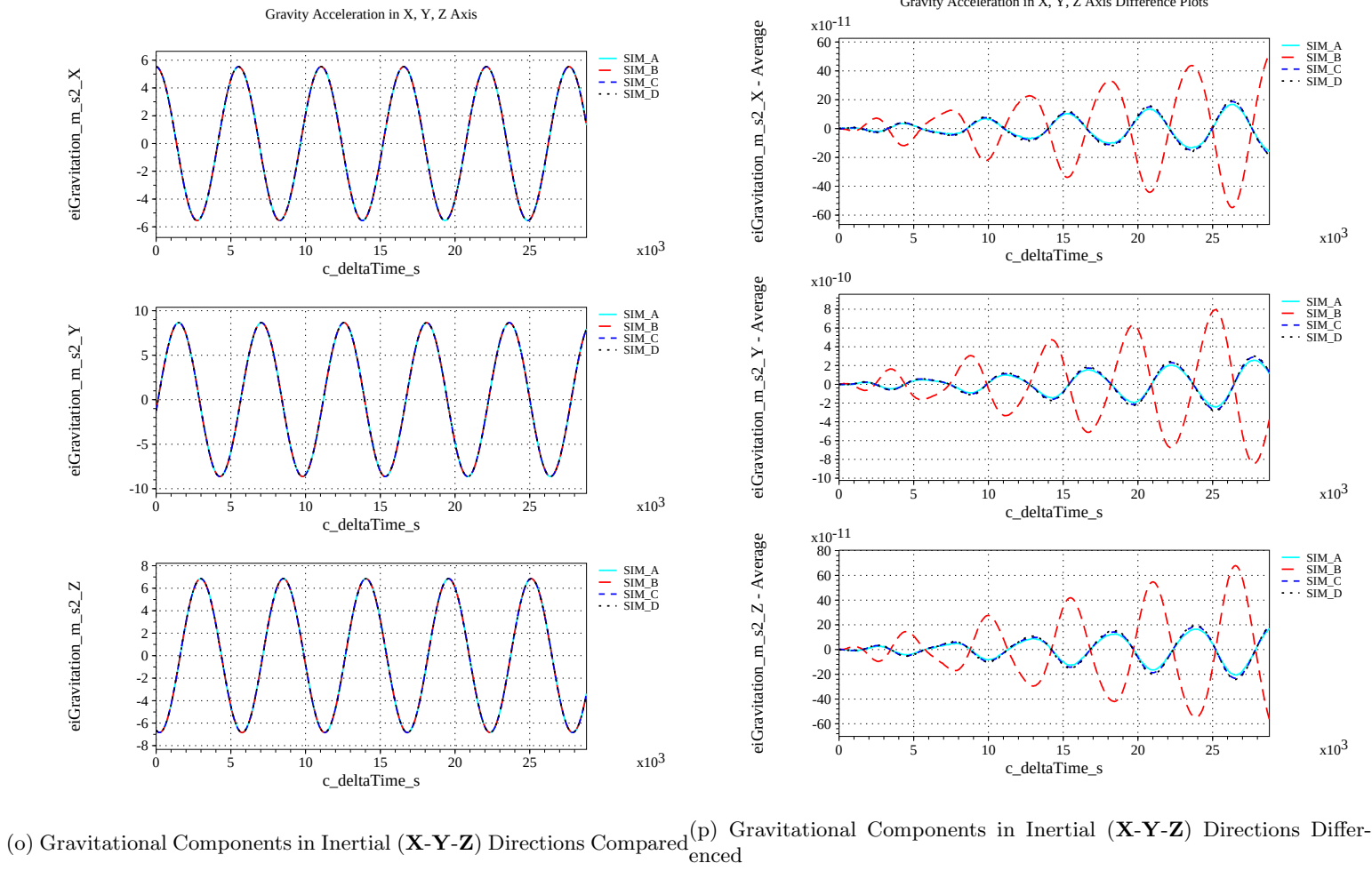
Figure 52. Check-case 08A: ISS Free Rotation with Zero Rates; See Discussion in Section D.2.16 (Concluded)
