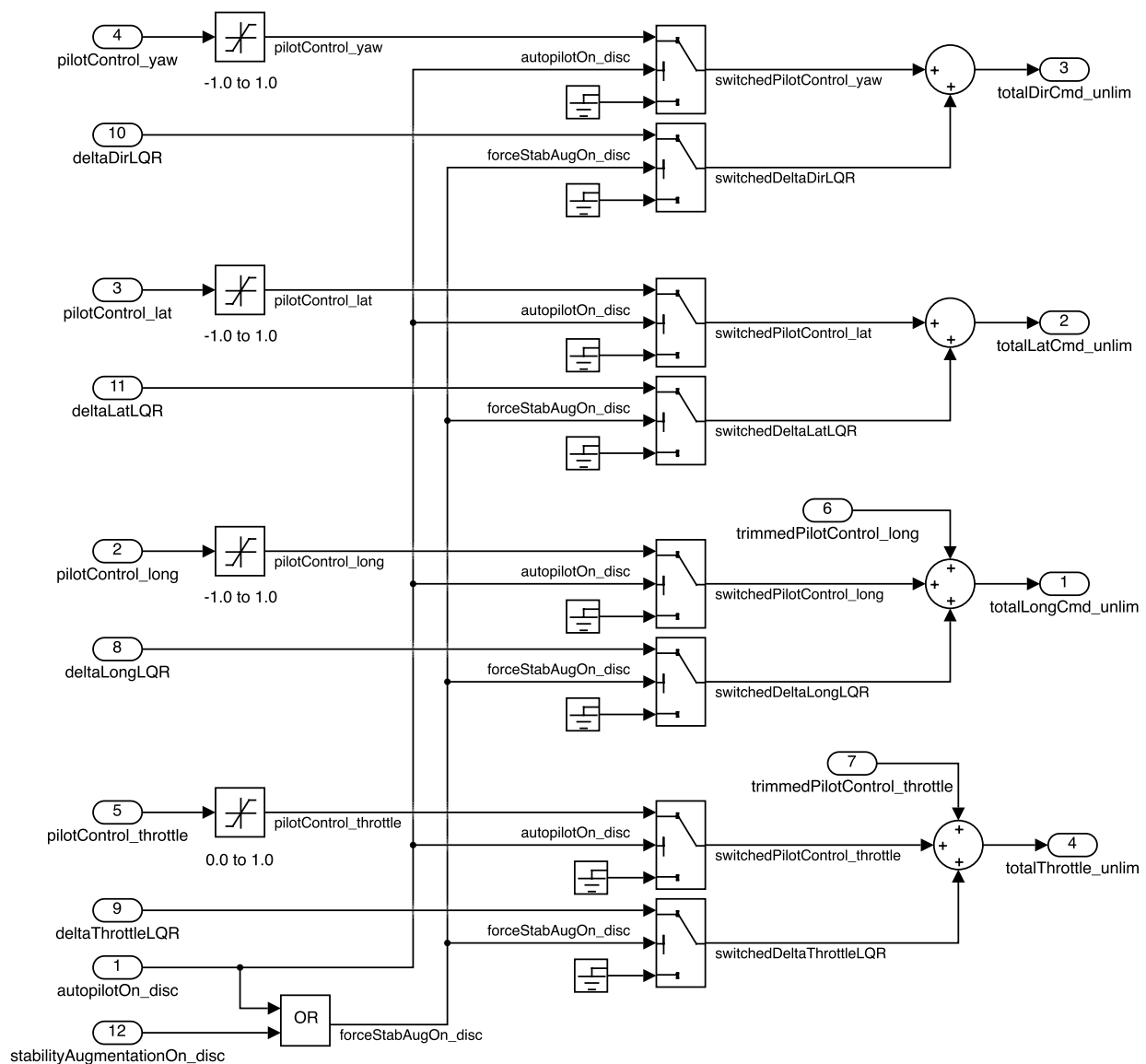
Figure 8. Engage logic: Select Sources to Drive Control Surfaces and Power Lever Angle
