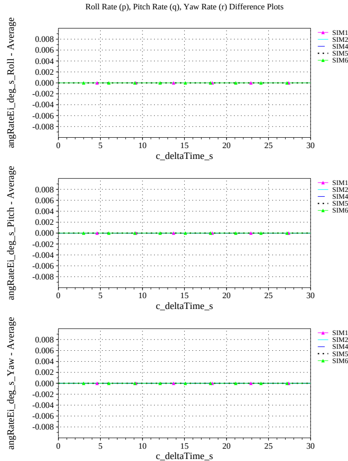
(r) Body-axis Angular Rates (w.r.t. NED Frame) Differenced
