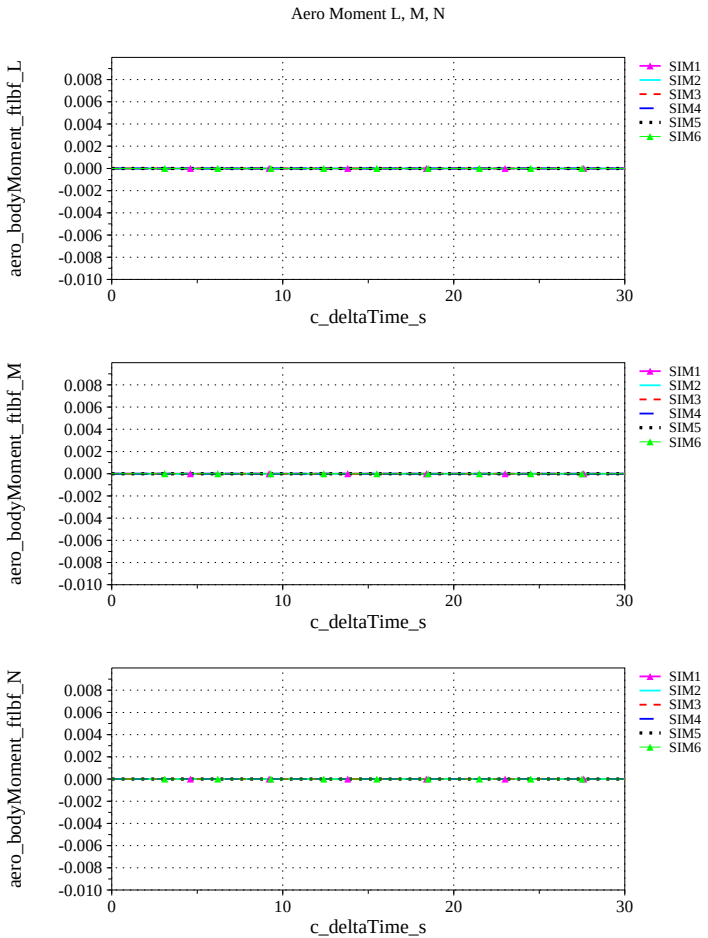
(c) Aerodynamic Moments Compared
