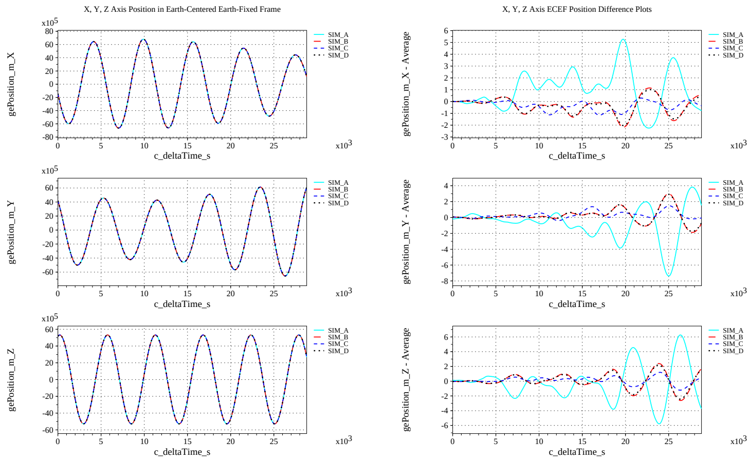
(k) Earth-centered, Earth-fixed Rectangular (X-Y-Z) Positions Compared (l) Earth-centered, Earth-fixed Rectangular (X-Y-Z) Positions Differenced
