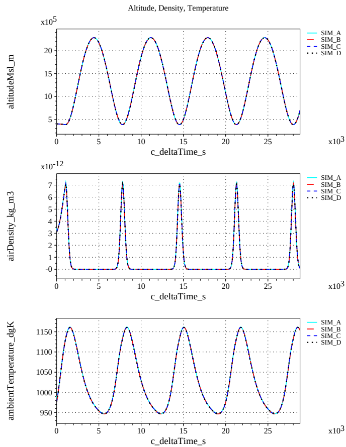
(c) Atmospheric Properties Compared
