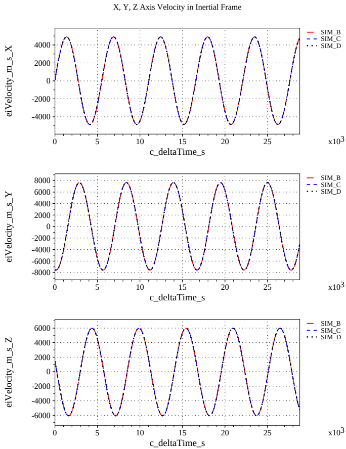
(g) Inertial Velocities Compared
