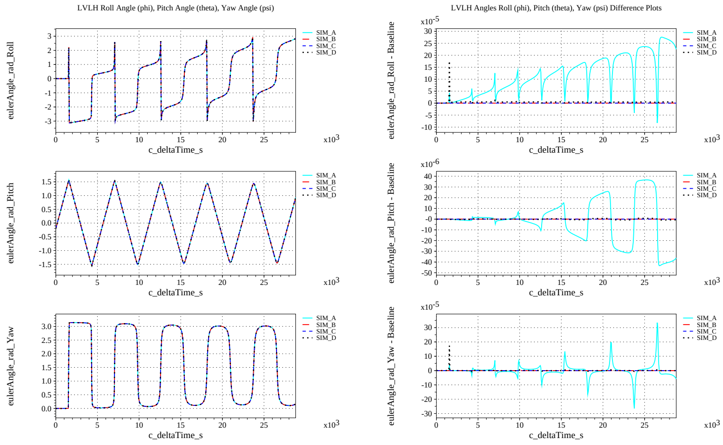
(i) Rotation Angles with Respect to LVLH Frame Compared (j) Rotation Angles with Respect to LVLH Frame Differenced
