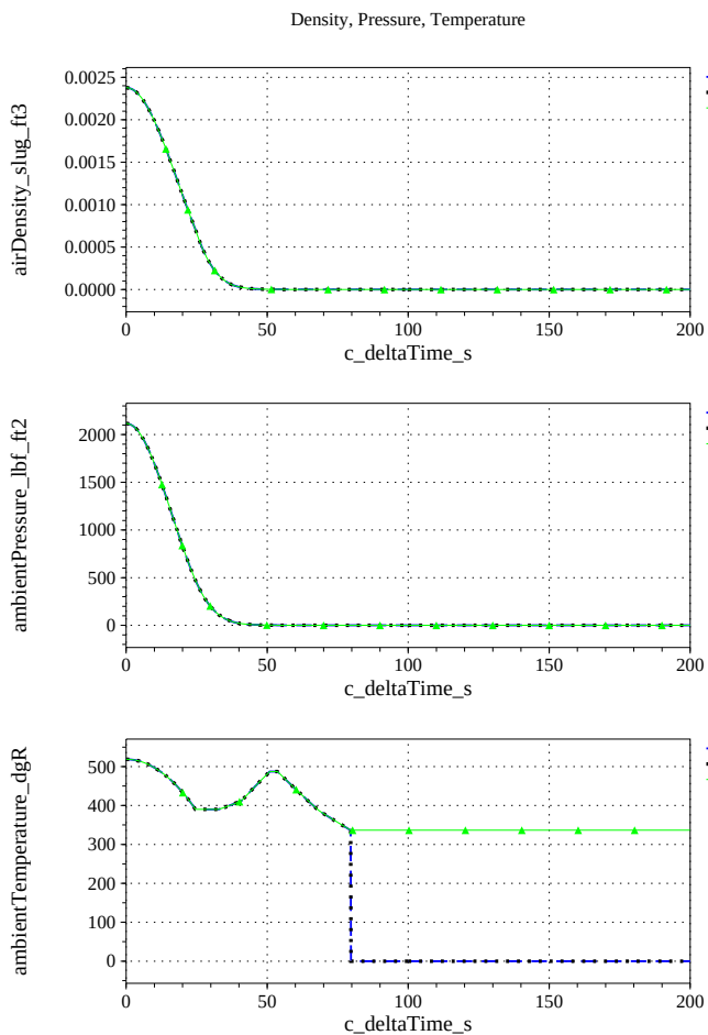
(s) Atmospheric Properties Compared
