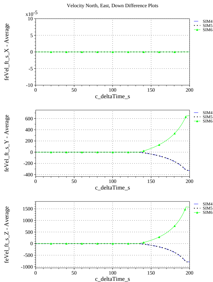
(n) NED Velocities Differenced
