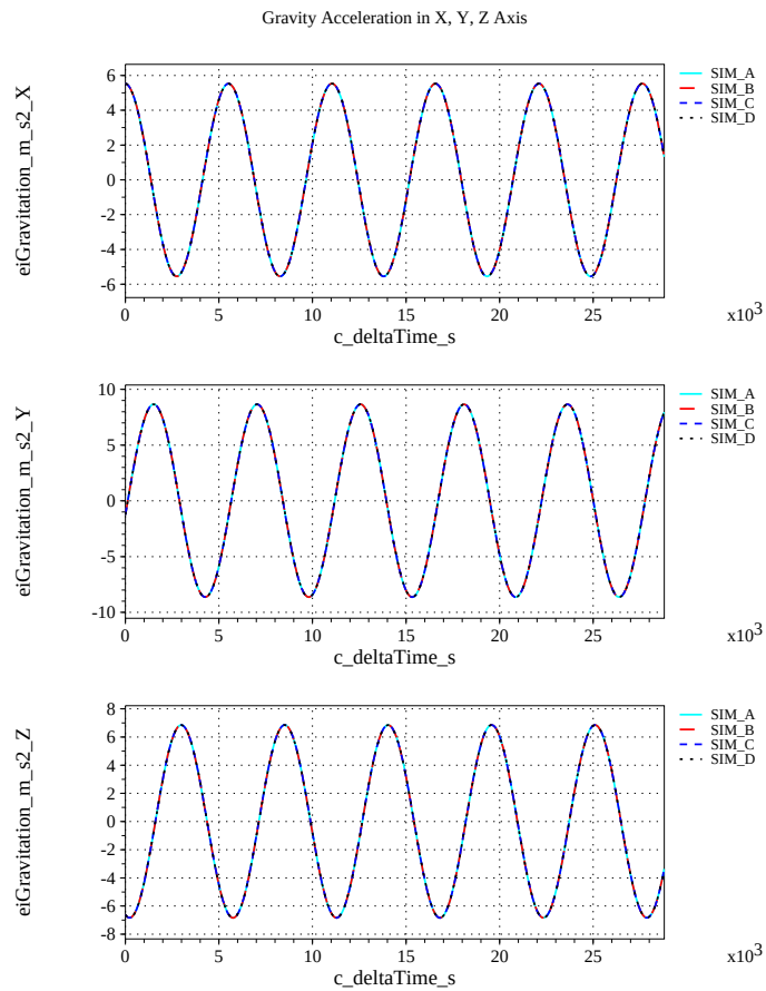
(o) Gravitational Components in Inertial ( X-Y-Z ) Directions Compared (p) Gravitational Components in Inertial ( X-Y-Z ) Directions Differenced
