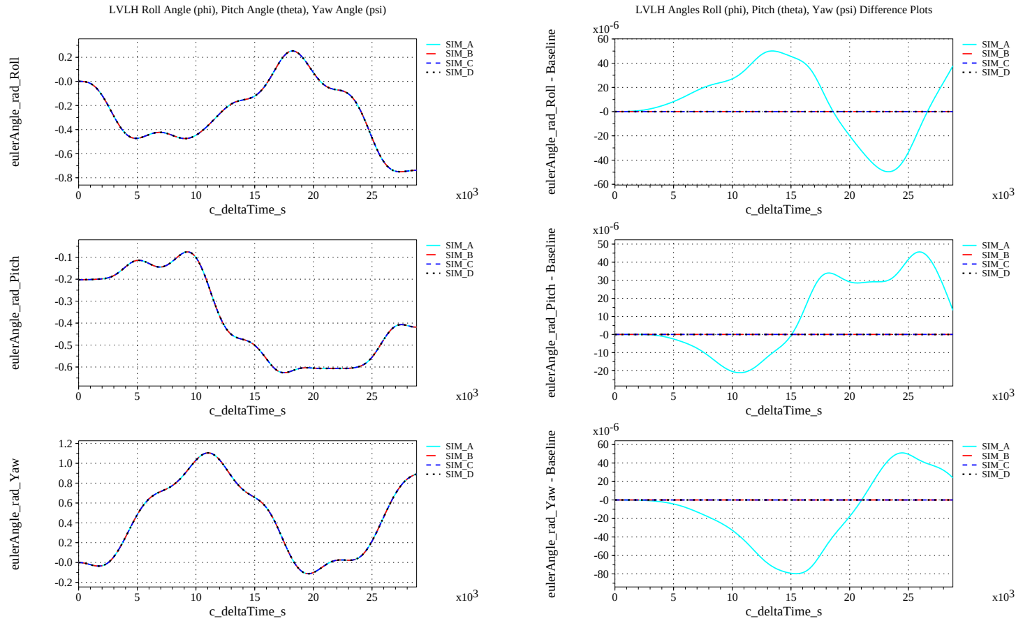
(i) Rotation Angles with Respect to LVLH Frame Compared
