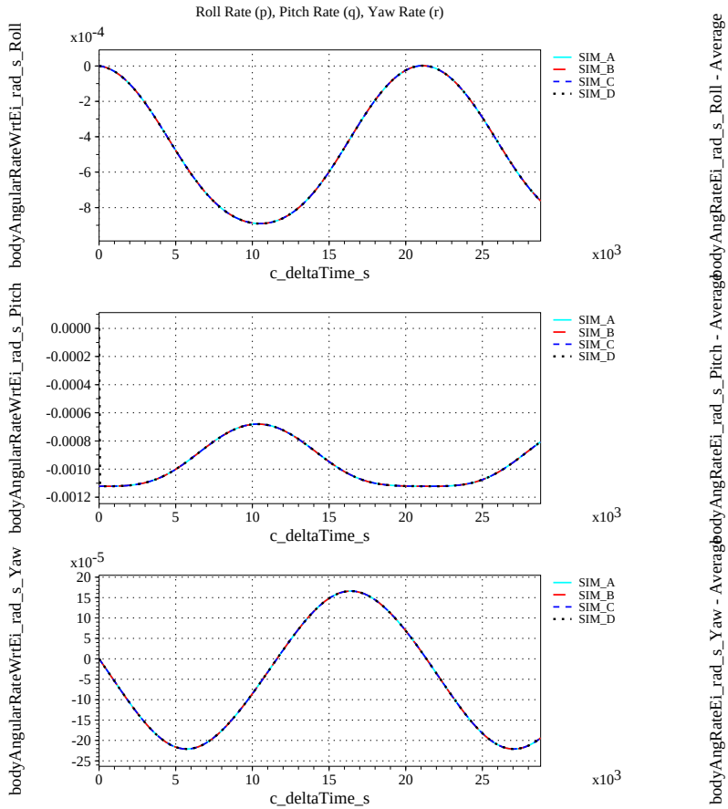
(e) Body-axis Angular Rates Compared
