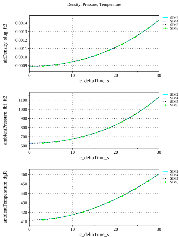
(s) Atmospheric Properties Compared
