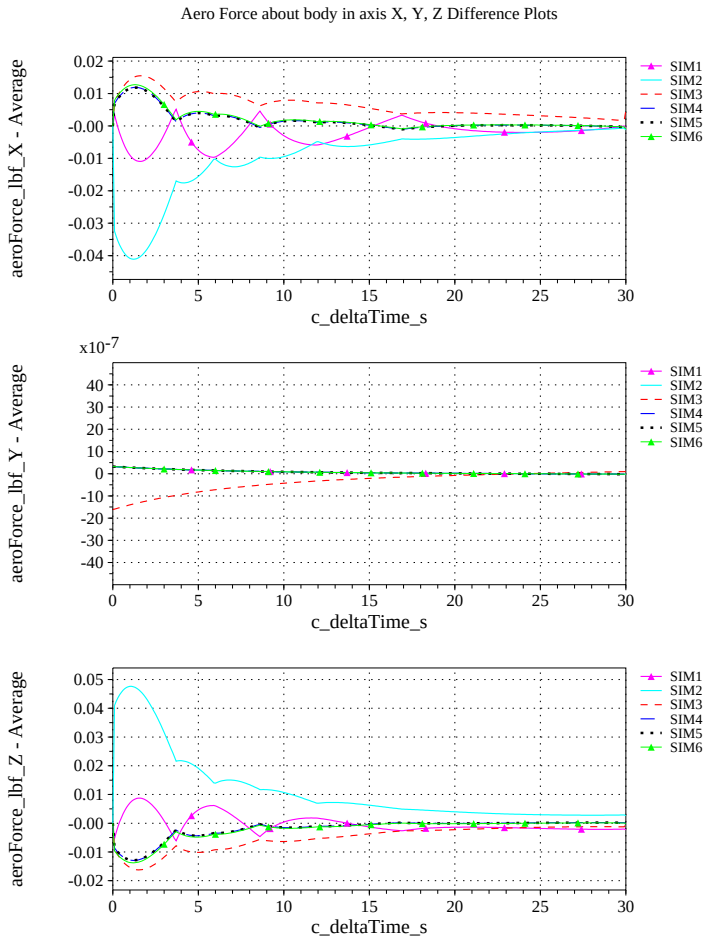
(b) Aerodynamic Forces Differenced
