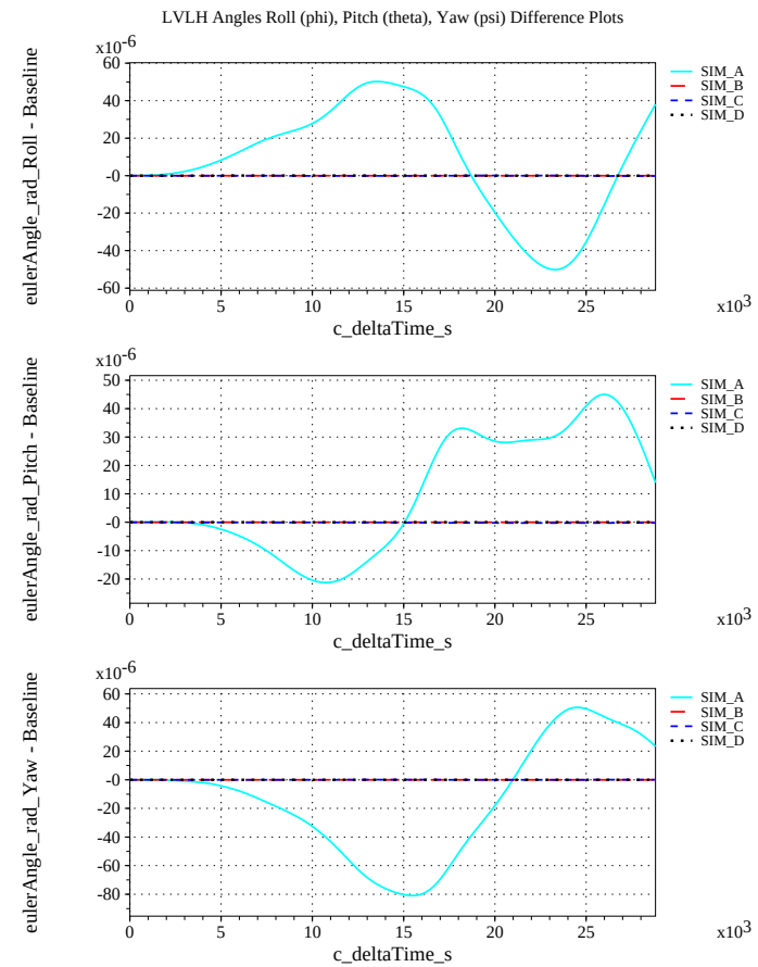
(j) Rotation Angles with Respect to LVLH Frame Differenced
