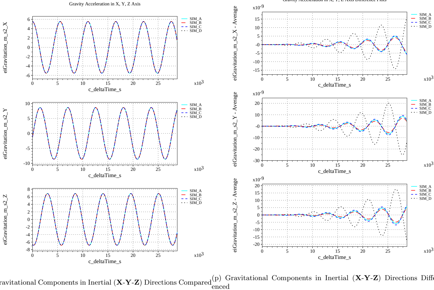
Figure 40. Check-case 04: ISS with Third-body Disturbances; See Discussion in Section D.2.4 (Concluded)
