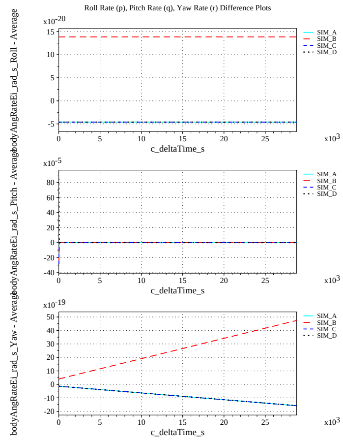
(f) Body-axis Angular Rates Differenced
