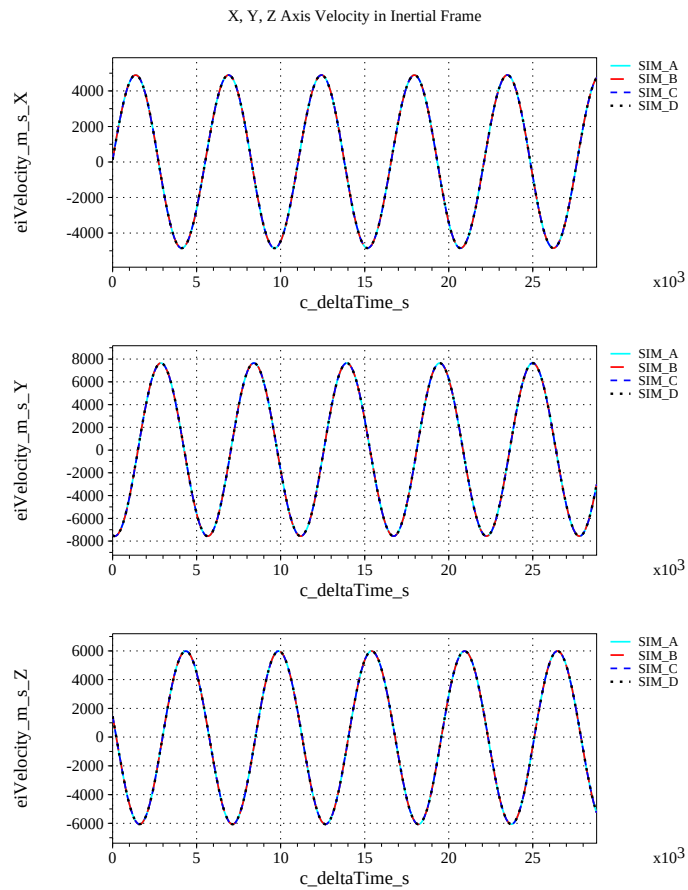
(g) Inertial Velocities Compared
