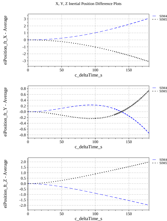
(x) Earth-centered Inertial Rectangular (x-y-z) Positions Differenced
