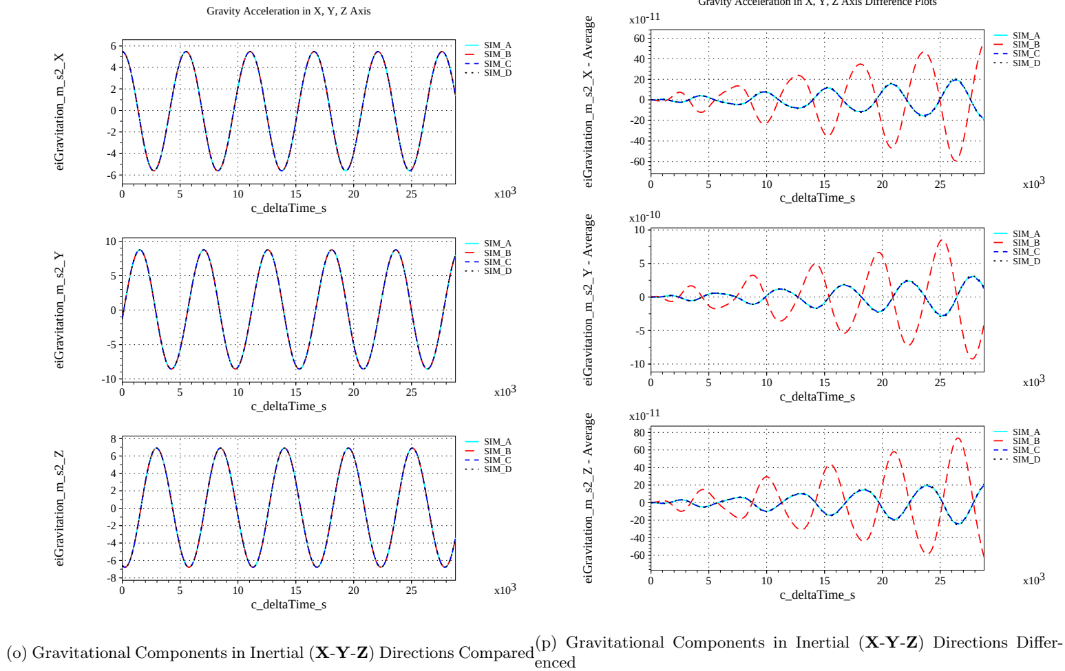
Figure 41. Check-case 05A: ISS (Minimal Solar Activity); See Discussion in Section D.2.5 (Concluded)
