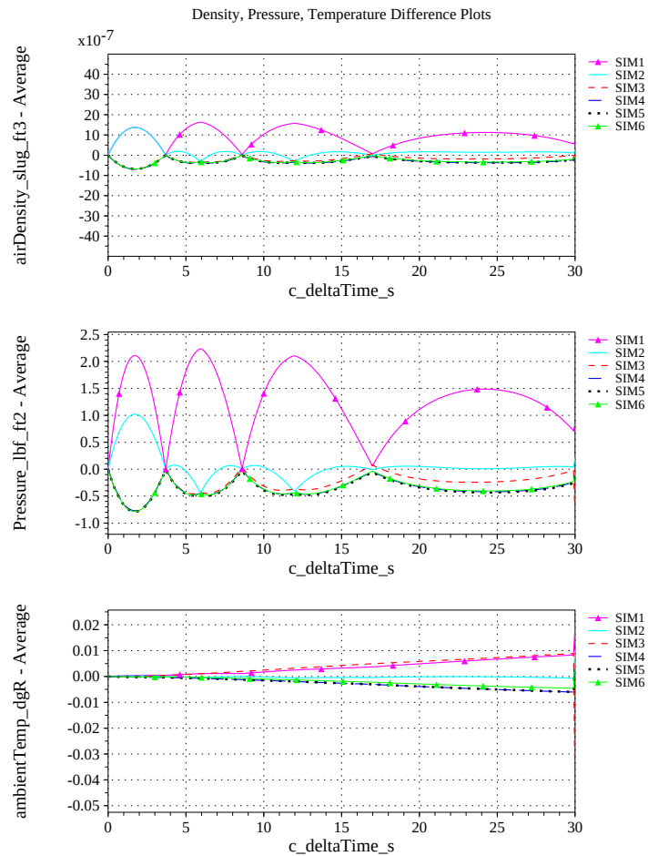
(t) Atmospheric Properties Differenced
