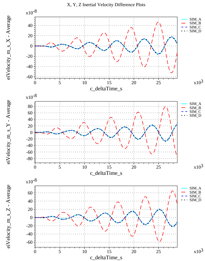
(h) Inertial Velocities Differenced
