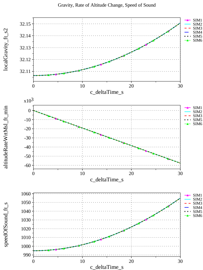
(i) Gravity, Climb Rate, and Speed-of-sound Compared
