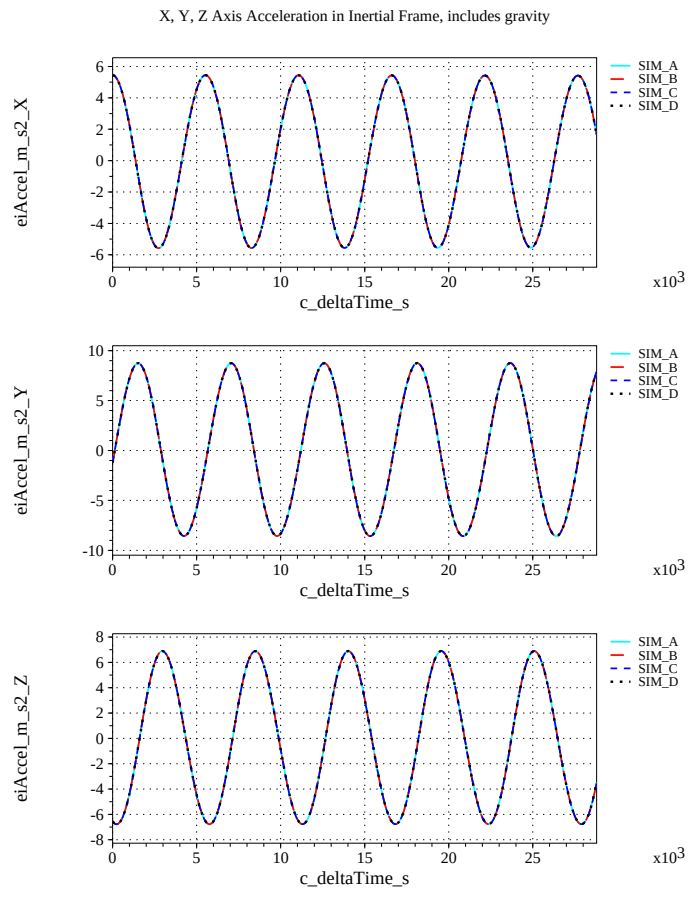
(a) Inertial Accelerations Compared
