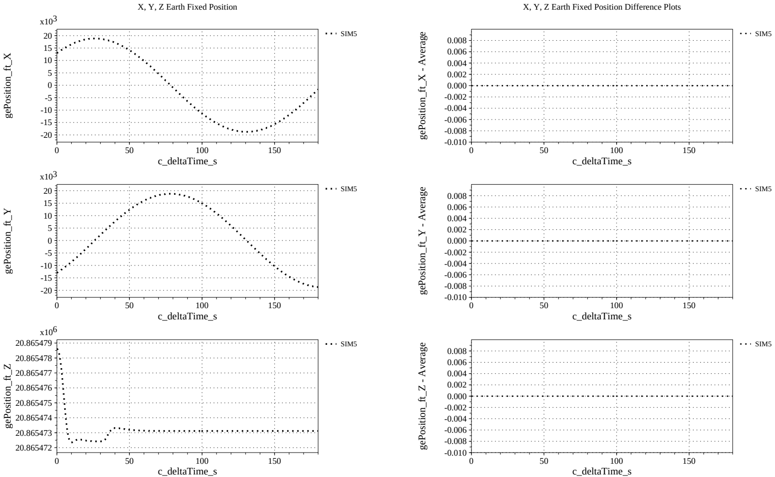
(u) Earth-centered, Earth-fixed Rectangular (X-Y-Z) Positions Compared (v) Earth-centered, Earth-fixed Rectangular (X-Y-Z) Positions Differenced
