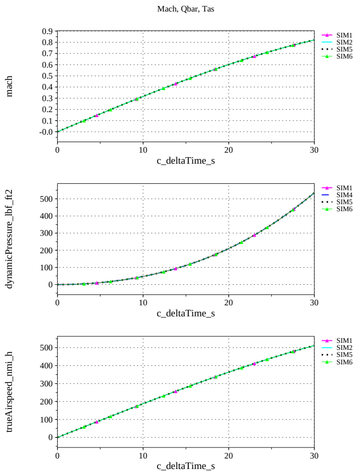
(k) Mach, Dynamic Pressure, and True Airspeed Compared
