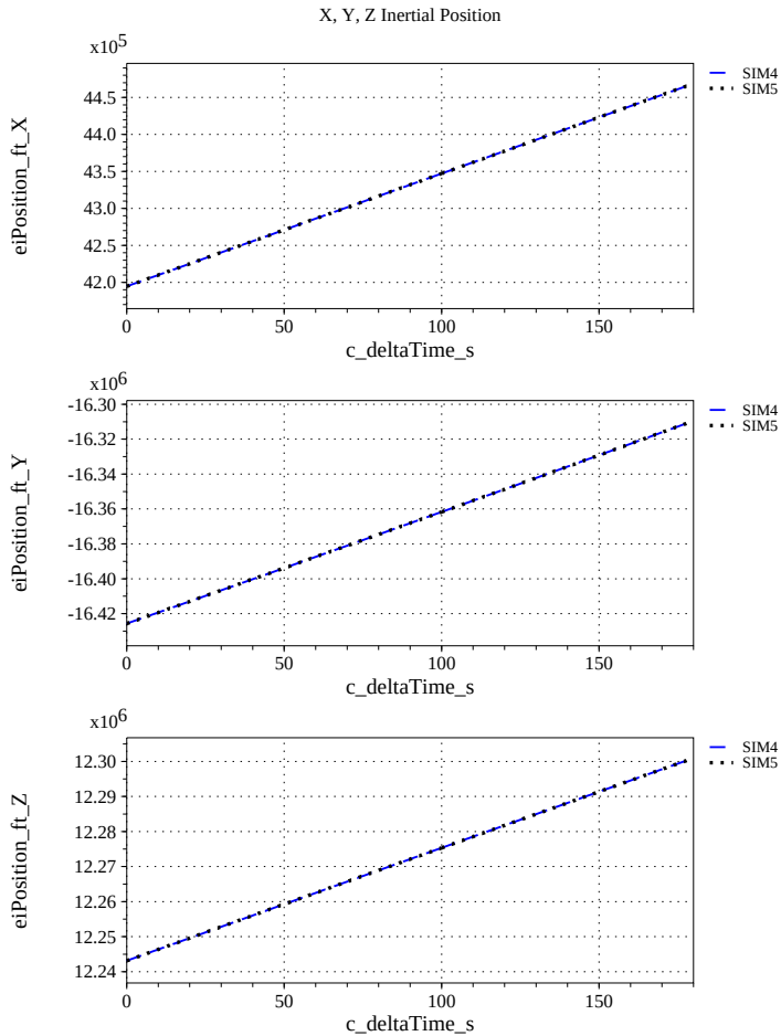
(w) Earth-centered Inertial Rectangular (x-y-z) Positions Compared
