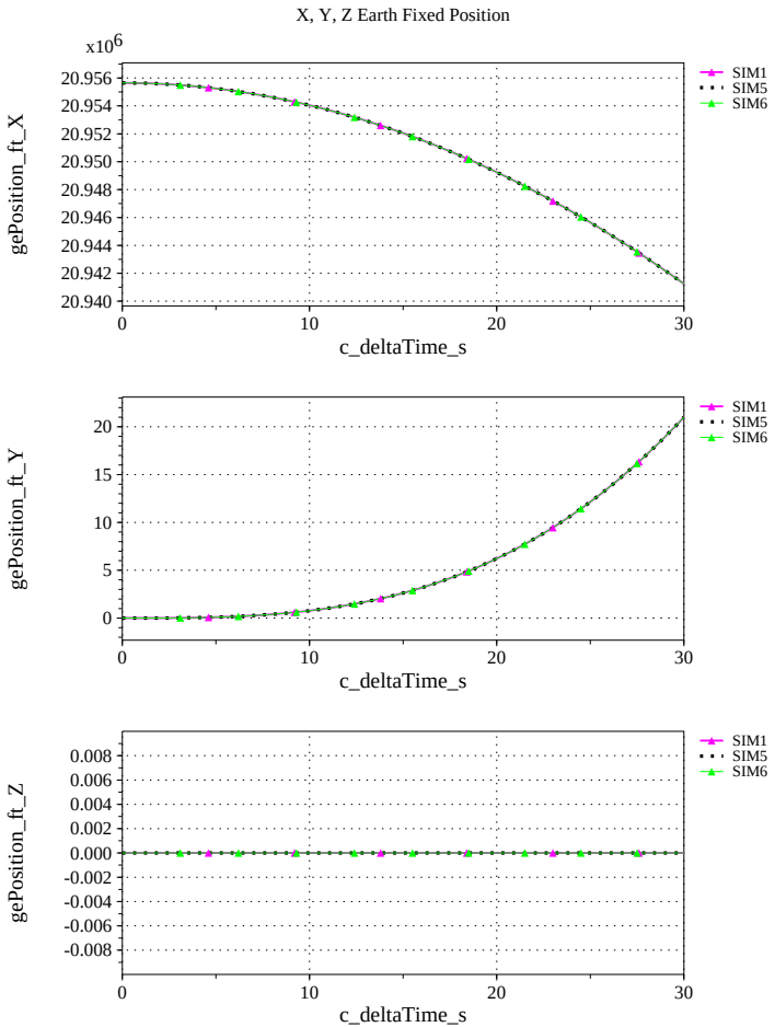
(u) Earth-centered, Earth-fixed Rectangular ( X - Y - Z ) Positions Compared (v) Earth-centered, Earth-fixed Rectangular ( X - Y - Z ) Positions Differenced
