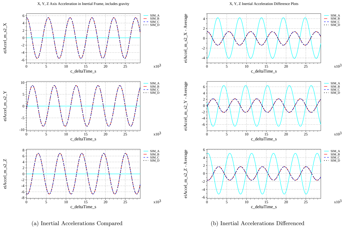
Figure 42. Check-case 05B: ISS (Mean Solar Activity); See Discussion in Section D.2.6
