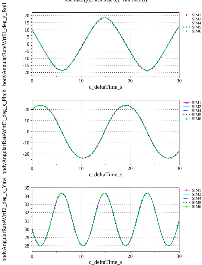
(q) Body-axis Angular Rates (w.r.t. NED Frame) Compared
