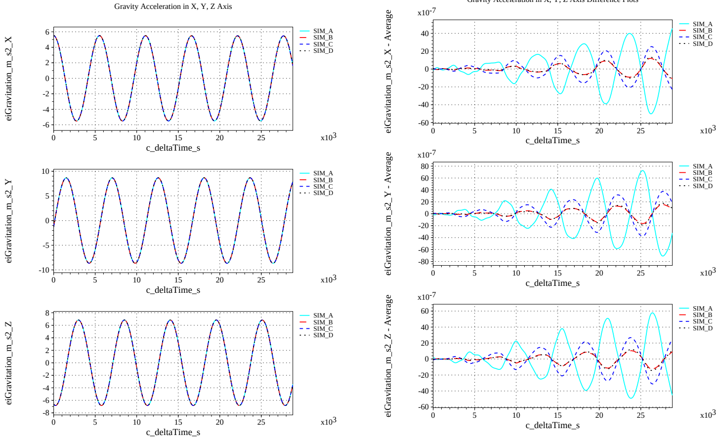
(o) Gravitational Components in Inertial (X-Y-Z) Directions Compared (p) Gravitational Components in Inertial (X-Y-Z) Directions Differ- enced
