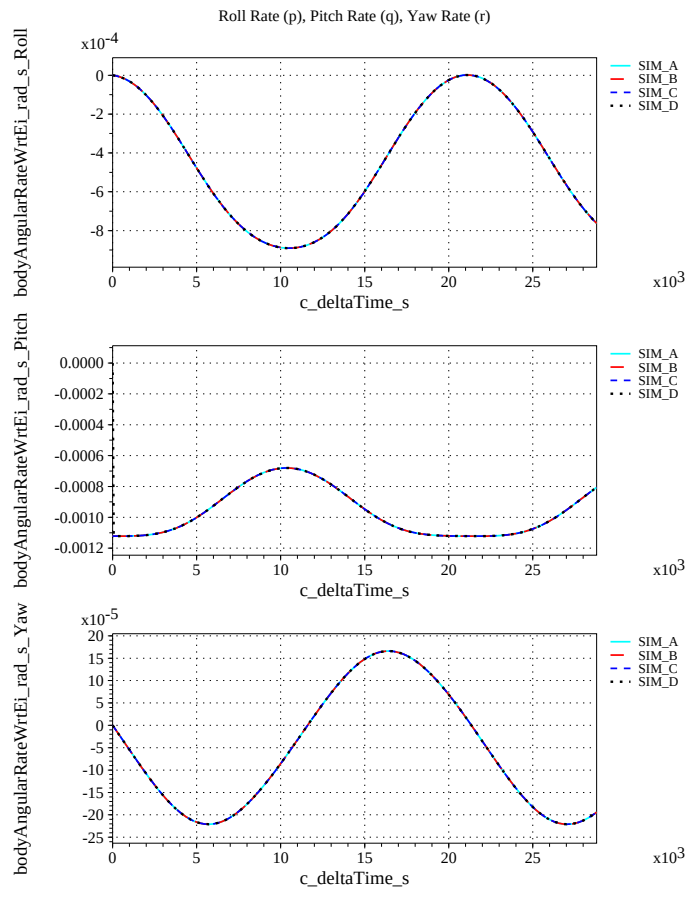
(e) Body-axis Angular Rates Compared
