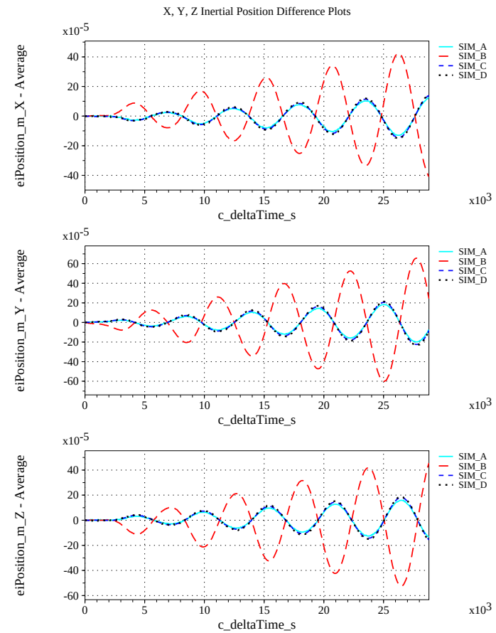
(m) Earth-centered Inertial Rectangular (x-y-z) Positions Compared (n) Earth-centered Inertial Rectangular (x-y-z) Positions Differenced
