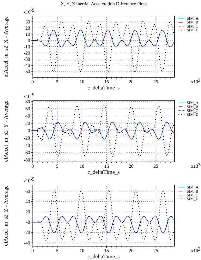
(b) Inertial Accelerations Differenced
