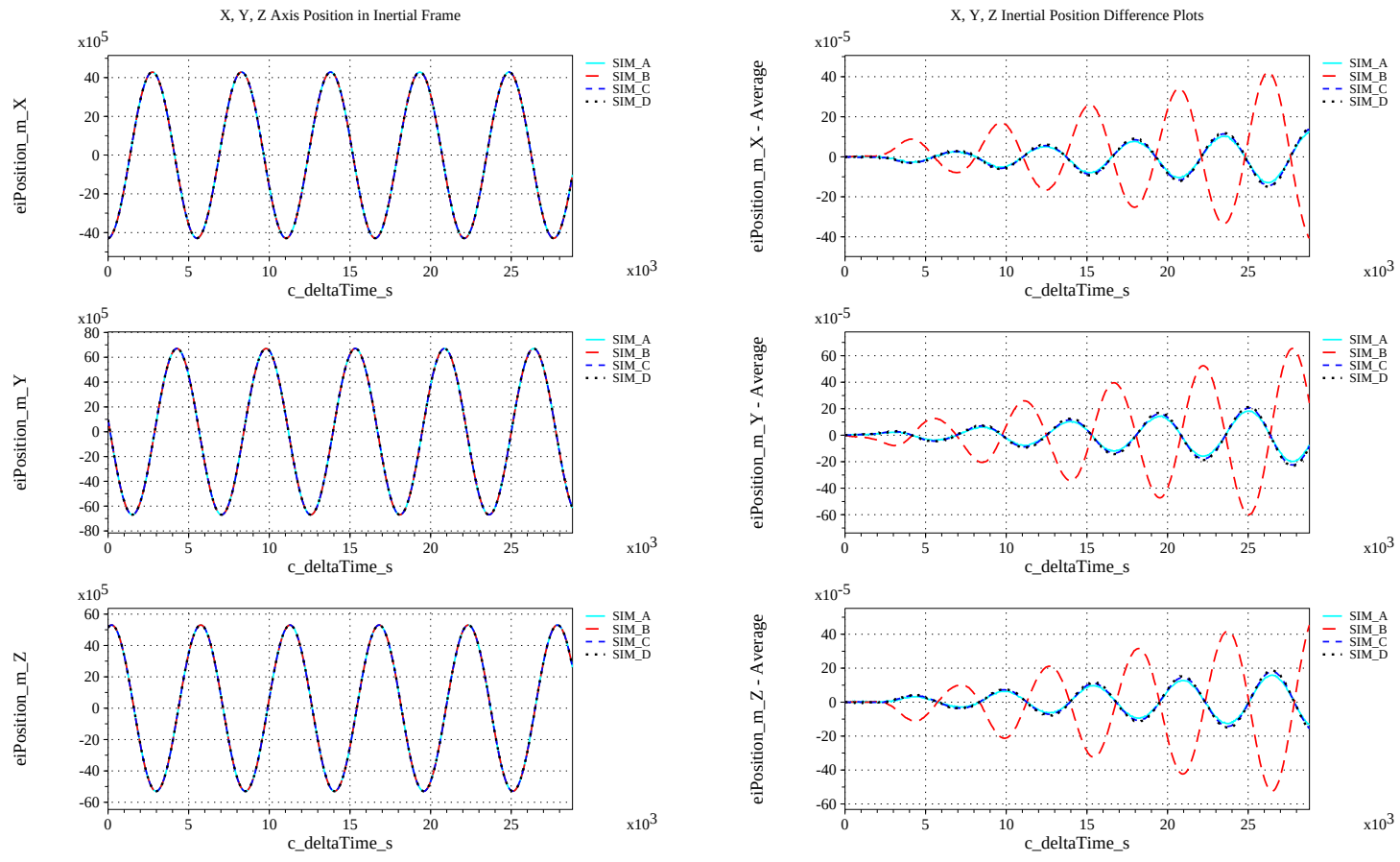
Figure 58. Check-case 10A: Cylinder in Circular Orbit with Gravity Gradient with Zero Initial Rates; See Discussion in Section D.2.22 (Cont'd)
