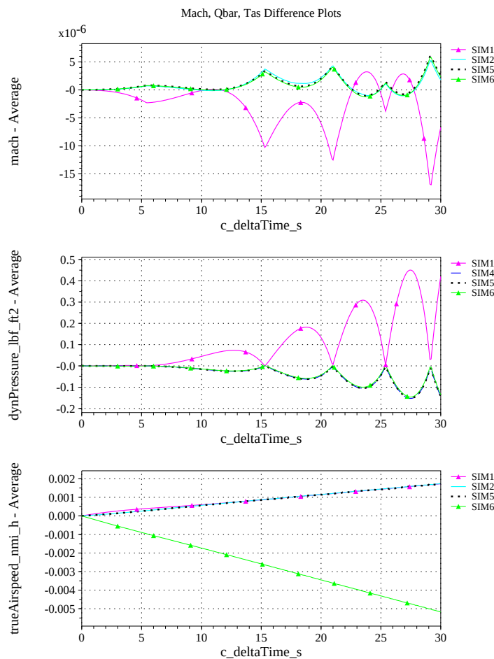
(l) Mach, Dynamic Pressure, and True Airspeed Differenced
