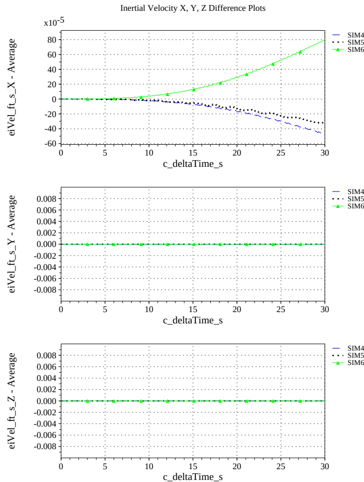
(p) Inertial Velocities Differenced
