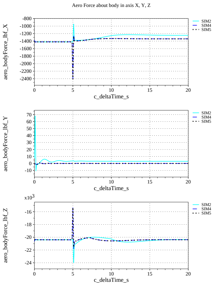
(a) Aerodynamic Forces Compared
