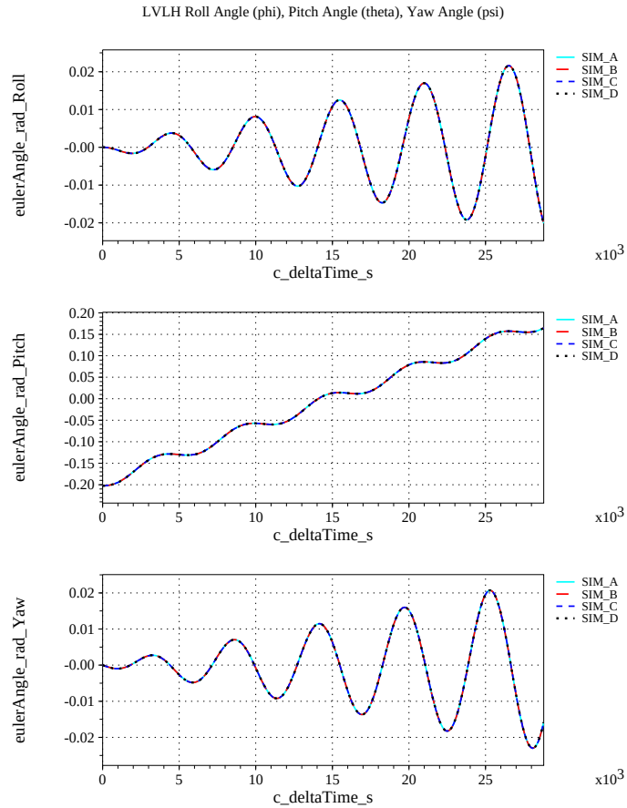
(i) Rotation Angles with Respect to LVLH Frame Compared
