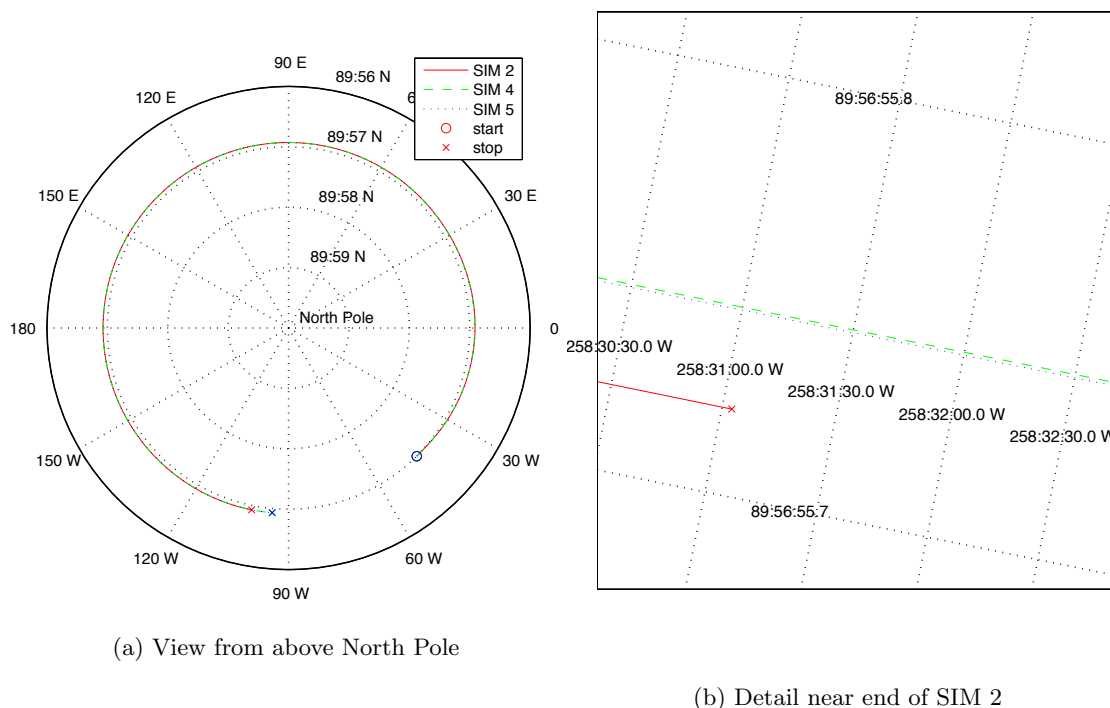
Figure 32. Trajectories of Simulated F-16 Circling the North Pole for Three Simulation Tools
