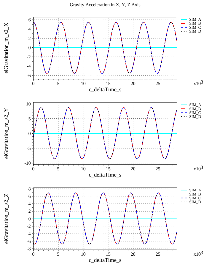
(o) Gravitational Components in Inertial (X-Y-Z) Directions Compared
