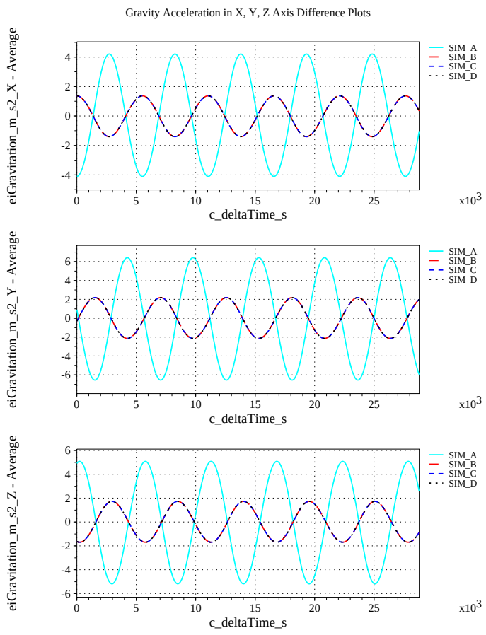
(p) Gravitational Components in Inertial (X-Y-Z) Directions Differ- enced
