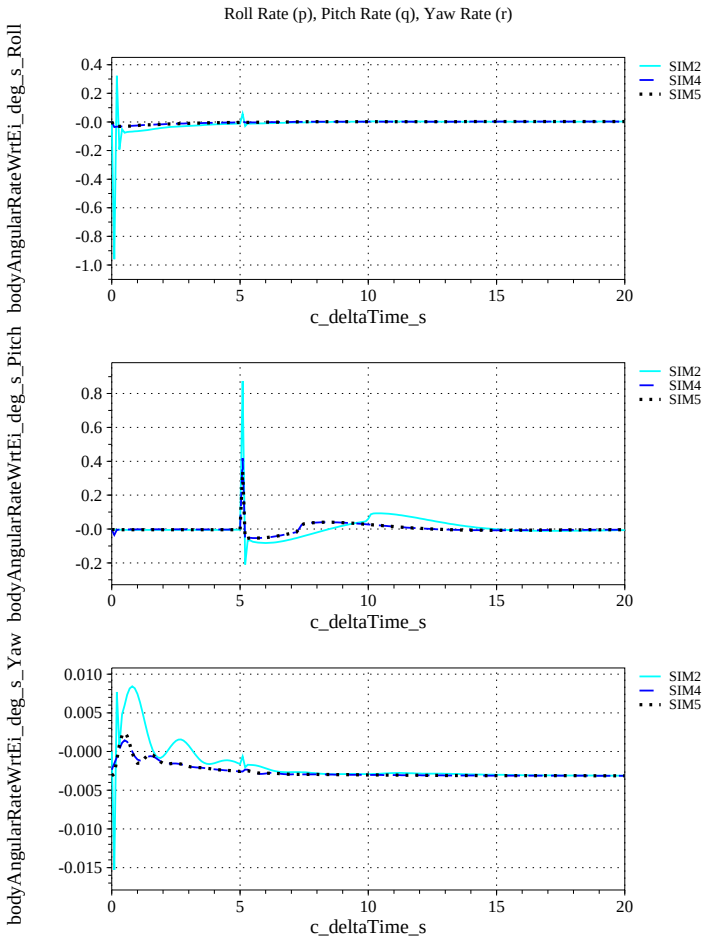
(q) Body-axis Angular Rates (w.r.t. NED Frame) Compared
