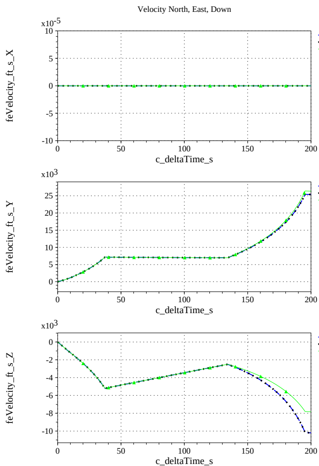
(m) NED Velocities Compared
