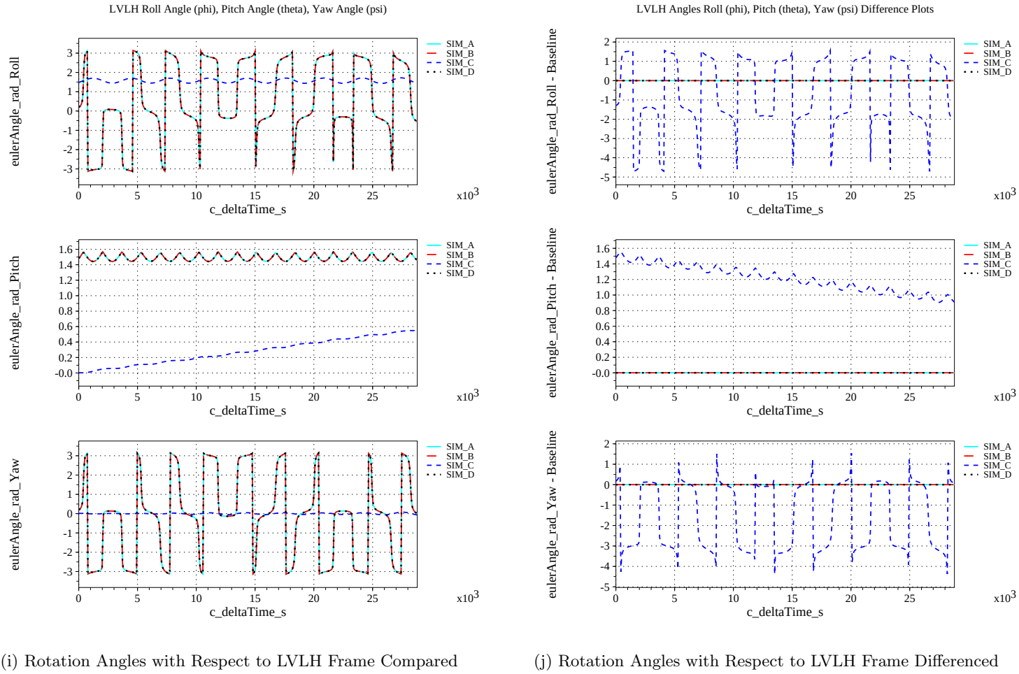
Figure 59. Check-case 10B: Cylinder in Circular Orbit with Gravity Gradient with Non-zero Initial Rates; See Discussion in Section D.2.23 (Cont'd)
