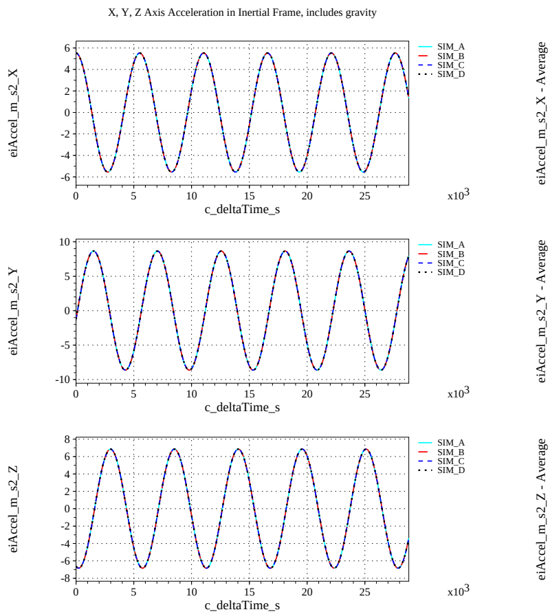
(a) Inertial Accelerations Compared
