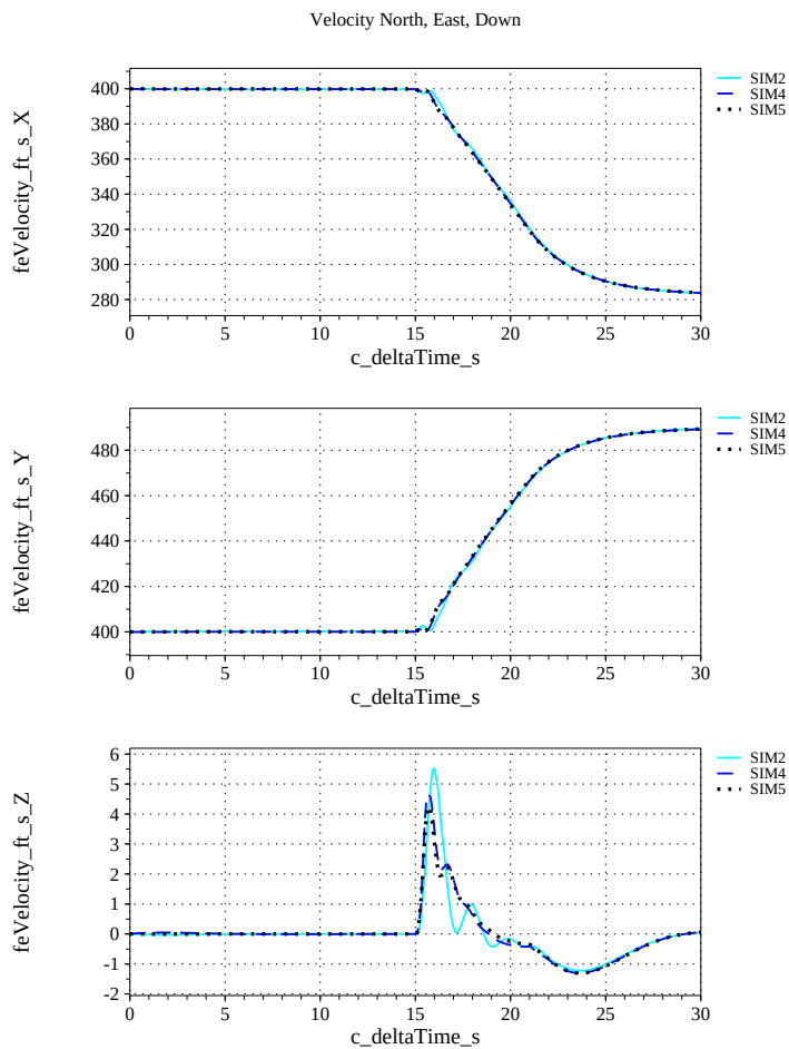
(m) NED Velocities Compared
