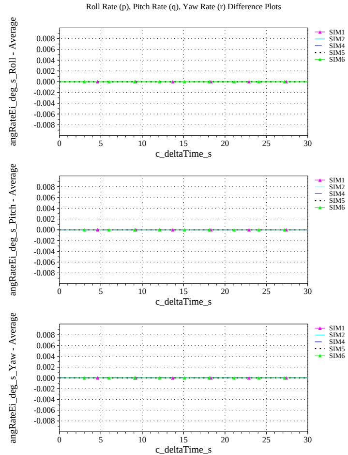
(r) Body-axis Angular Rates (w.r.t. NED Frame) Differenced
