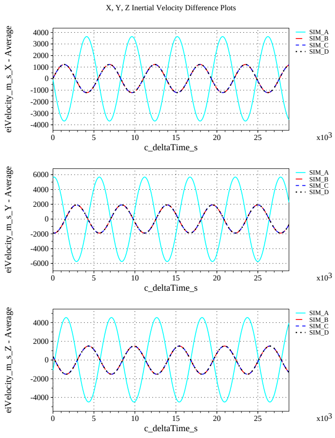
(h) Inertial Velocities Differenced
