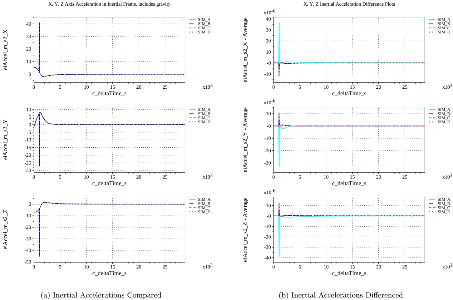
Figure 47. Check-case 06D: Cylinder Undergoing Earth Departure Firing; See Discussion in Section D.2.11
