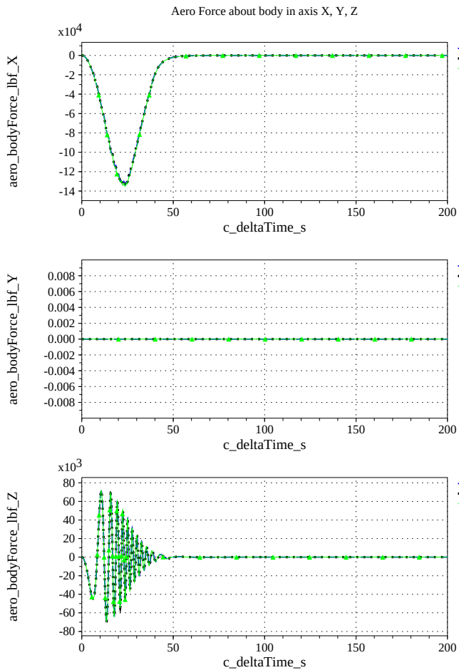
(a) Aerodynamic Forces Compared
