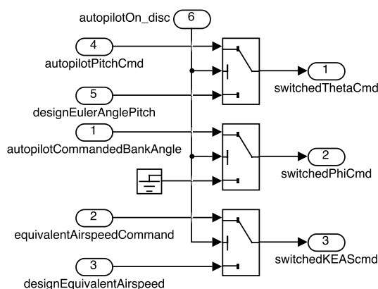
Figure 5. LQR input selection : Select Between Trimmed and Commanded Pitch, Roll, and Airspeed LQR Reference Inputs
