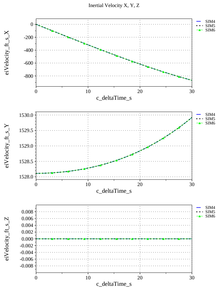
(o) Inertial Velocities Compared
