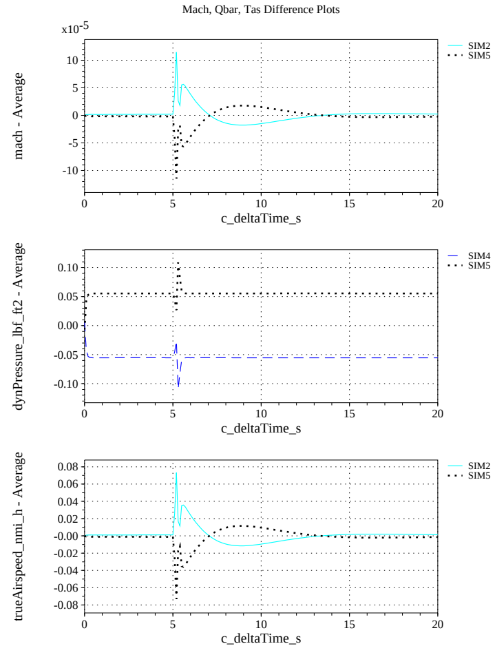
(l) Mach, Dynamic Pressure, and True Airspeed Differenced
