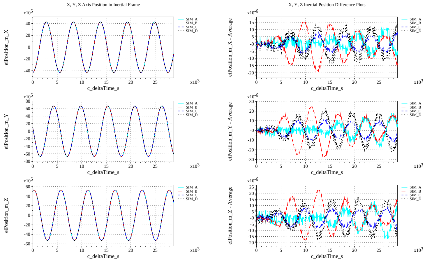
(m) Earth-centered Inertial Rectangular (x-y-z) Positions Compared (n) Earth-centered Inertial Rectangular (x-y-z) Positions Differenced
