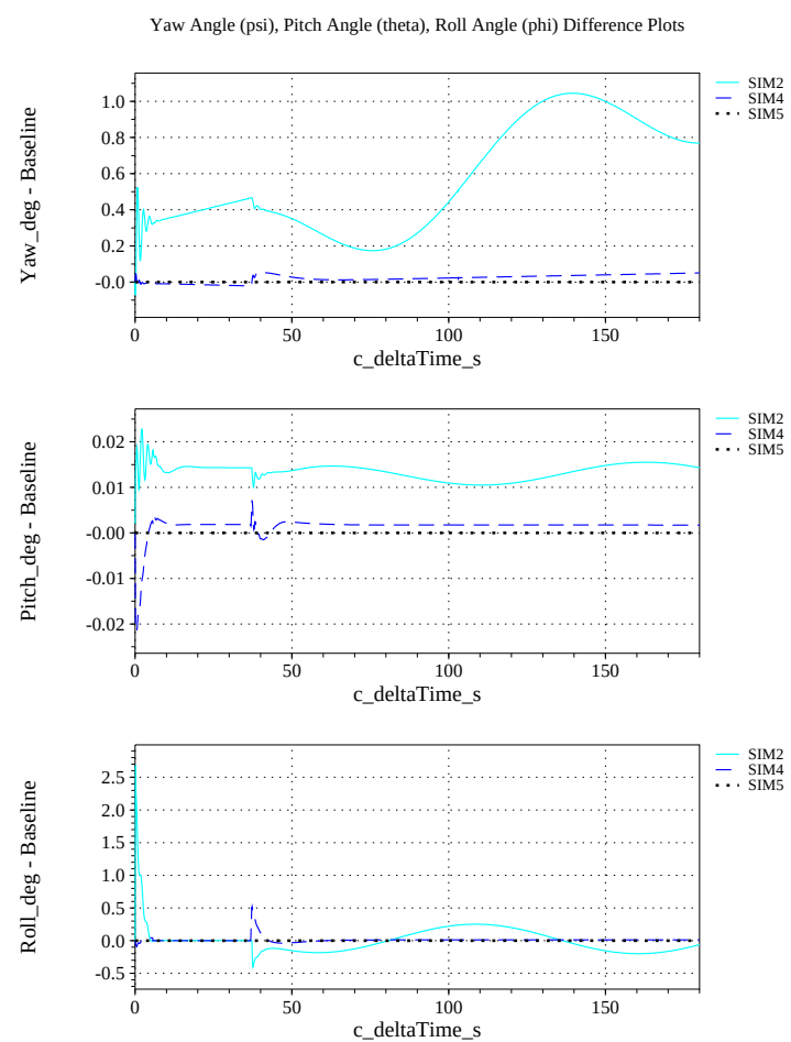
(h) Euler Angles (w.r.t. NED Frame) Differenced
