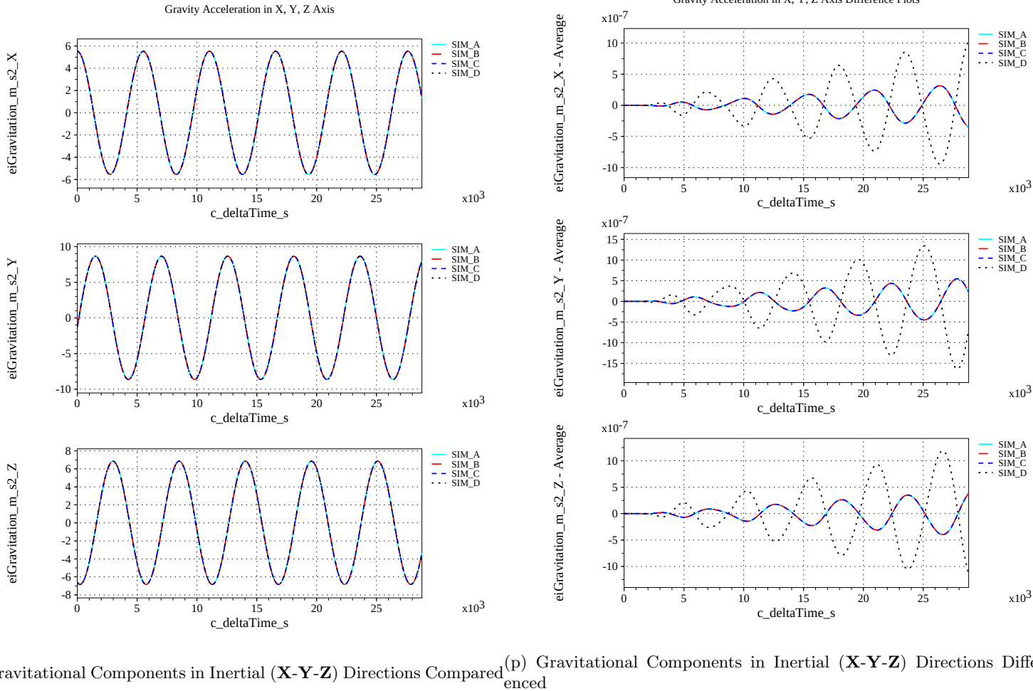
Figure 57. Check-case 09D: ISS Under Torque and Force with Non-zero Initial Rates; See Discussion in Section D.2.21 (Concluded)
