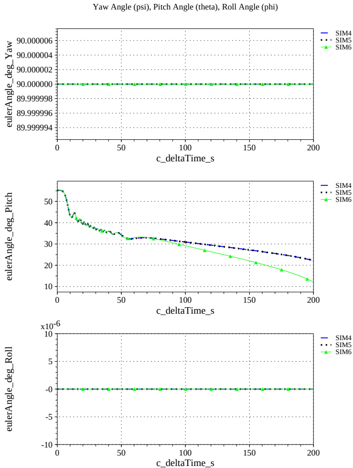
(g) Euler Angles (w.r.t. NED Frame) Compared
