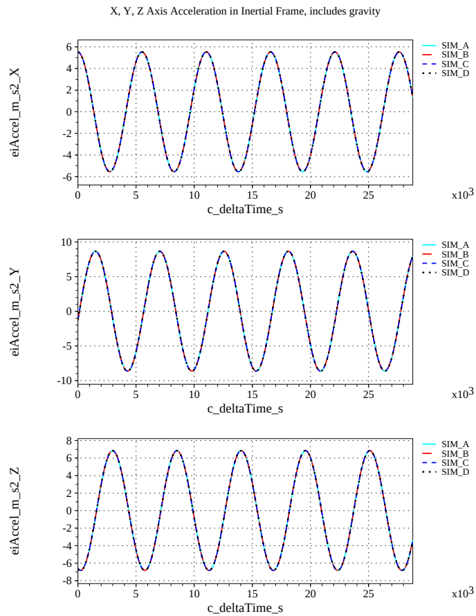
(a) Inertial Accelerations Compared
