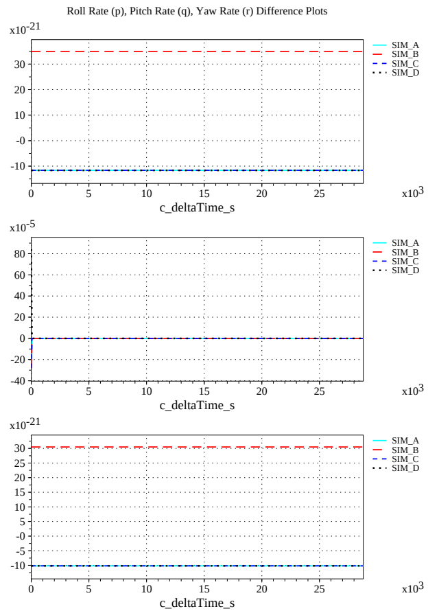
(f) Body-axis Angular Rates Differenced
