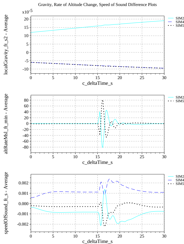
(j) Gravity, Climb Rate, and Speed-of-sound Differenced
