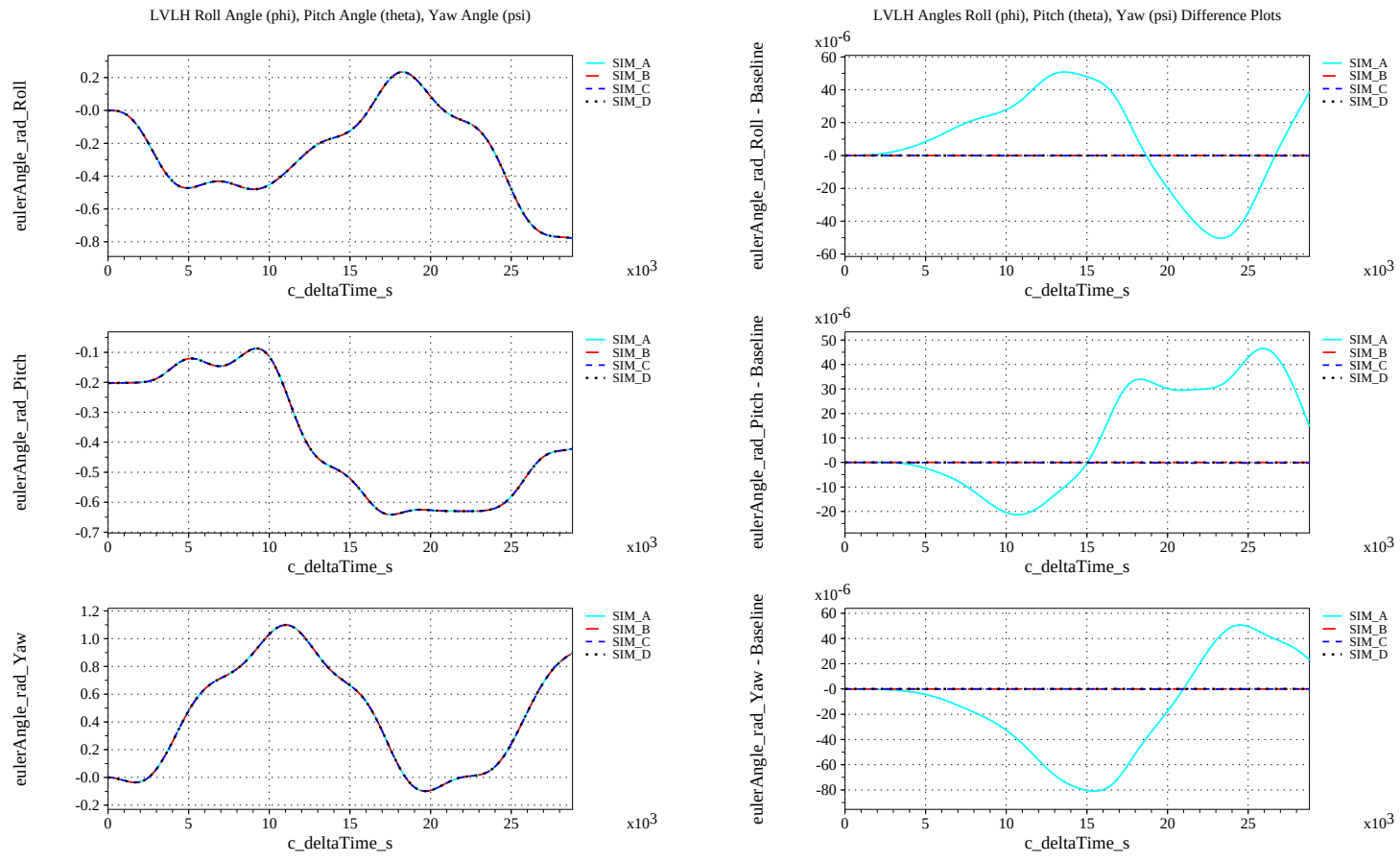
Figure 38. Check-case 03A: ISS in 4 \times 4 Harmonic Gravity; See Discussion in Section D.2.2 (Cont'd)
