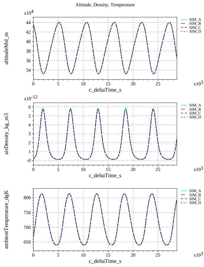
(c) Atmospheric Properties Compared
