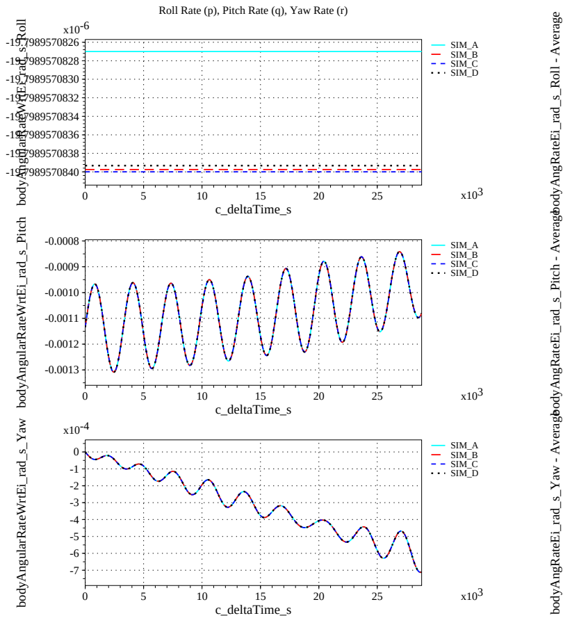
(e) Body-axis Angular Rates Compared
