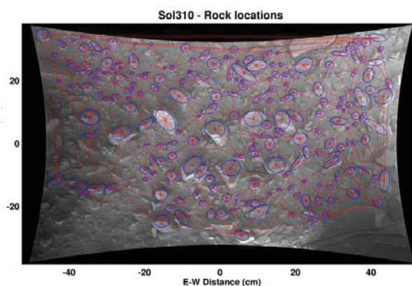
Figure 3: Delauney Triangulation (DT) analysis of the 217 clasts measured in the size frequency analysis of the MARDI twilight image acquired on Sol 310. The mean spacing between clasts (from DT analysis) is 5.1 cm, with a Mean/Std. Deviation (“Spacing Index”) of 1.54, which is a relatively common value for the 35 sites in Gale crater for which this type of analysis has been conducted.
