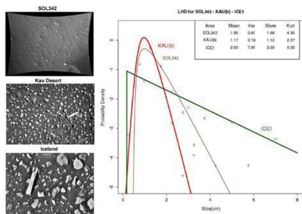
Figure 2: Comparison of hyperbolic clast size distributions for Sol 342 (Gale Crater) and those from two terrestrial reference sites: Kau desert (Hawaii) accidental debris and Icelandic sub-glacial debris near Askja caldera. Note the similarity between the distributions at Kau and Sol 342 and the contrast with the more poorly sorted Icelandic site. Development of a simple model to explain the evolution of such distributions is underway for the gravel sites on Mars.
