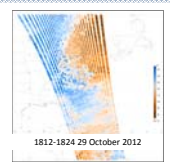
Figure 13. AIRS Ozone Anomaly
