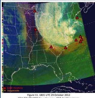
Figure 11. 1801 UTC 29 October 2012 CIRA/SPORT GOES Sounder proxy RGB Air Mass image
