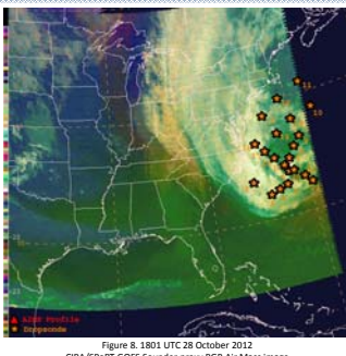
Figure 8. 1801 UTC 28 October 2012 CIRA/SPORT GOES Sounder proxy RGB Air Mass image
