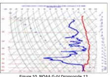
Figure 10. NOAA G-IV Dropsonde 12
