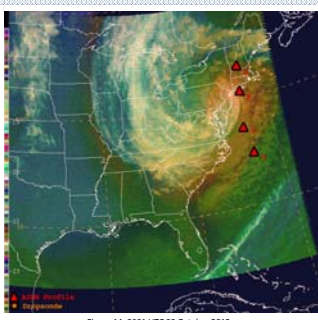
Figure 14. 0601 UTC 30 October 2012 CIRA/SPORT GOES Sounder proxy RGB Air Mass image
