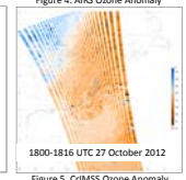
Figure 5. CrIMSS Ozone Anomaly
