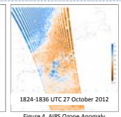
Figure 4. AIRS Ozone Anomaly
