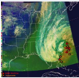
Figure 1. 1801 UTC 27 October 2012 CIRA/SPORT GOES Sounder proxy RGB Air Mass image
