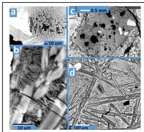
Figure 2. BSE images of shock melt vein materials in Kaidun. (a) & (b) From the CM1 lithology, serpentinite faithfully pseudomorphs a vein originally consisting of zoned, acicular olivine crystals nucleating into pyroxene composition mesostasis. (c) & (d) A fragment of a vein, still fresh, consisting of acicular plagioclase ( An_{22}Ab_{76}Or_2 ) nucleating into augite mesostasis (mainly Fs_{22}Wo_{36} ). After [5].
