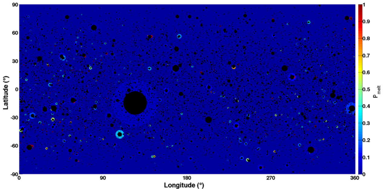
Figure 1: Post-bombardment distribution of impact-melt on Mars from a single impact history. The colors represent P_{melt} . Crater floors, where mass-wasting, which is not included in the model, likely modifies the composition, are denoted by black.
