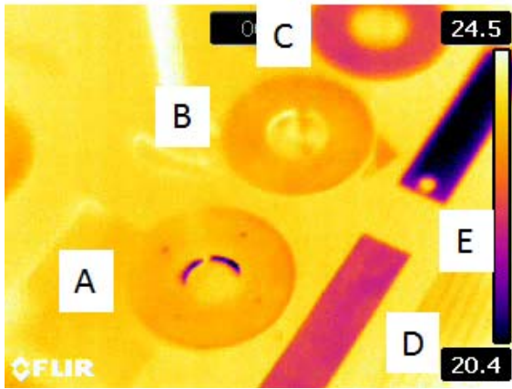
Figure 12: Comparison of the Thermal Contrast between AZ-93 Paint and Various Black Materials in the Shade
