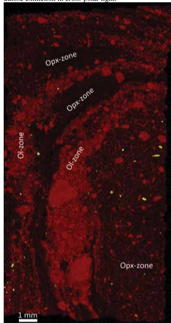
■ Olivine ■ Opx ■ Spinel ■ Sulfide Fig. 1: EDX map of thin section of NWA 5480
