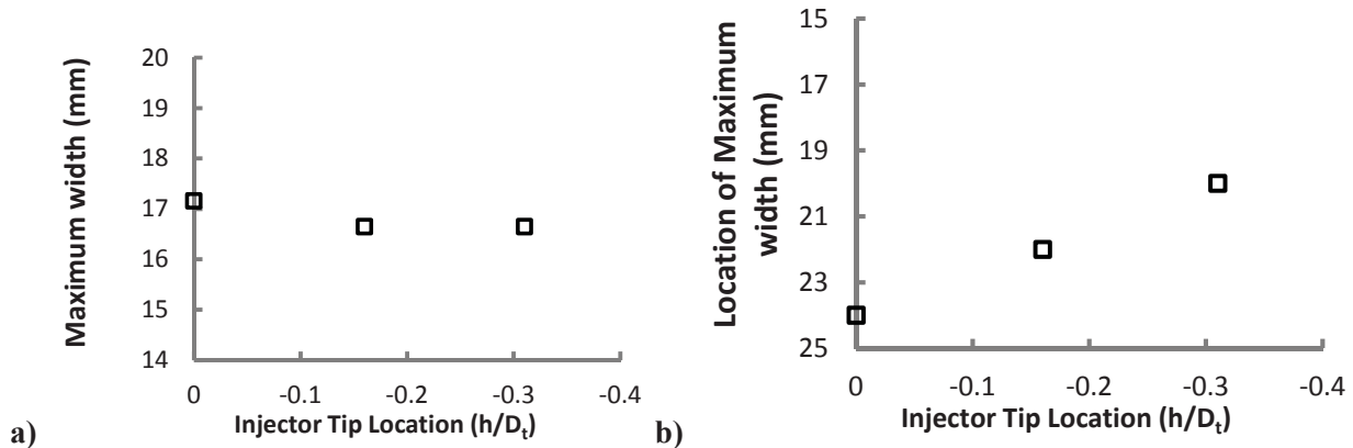
a) b) Figure 17.—Measures of Recirculation Zone Size. a) Plot of maximum width versus injector tip location diameter upstream of throat. b) Plot of location of maximum width versus injector tip location. Swirler angle 60^\circ and test condition 500.
