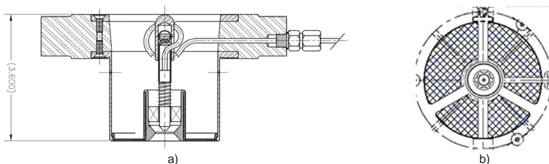
Figure 4.—Cross section of the single SV-LDI module. Detailed drawings showing a cross section of the single SV-LDI module in its spool piece; (a) and a bottom view that shows the screen inserted around the module (b).
