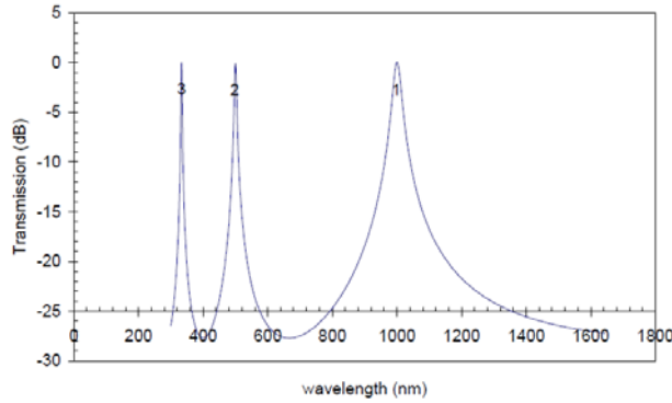
Figure 15. Spectral Transmission of Fabry Perot Etalons.
