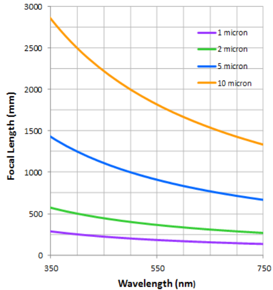
Figure 3. Optical Sieve plot of focal length versus wavelength.
