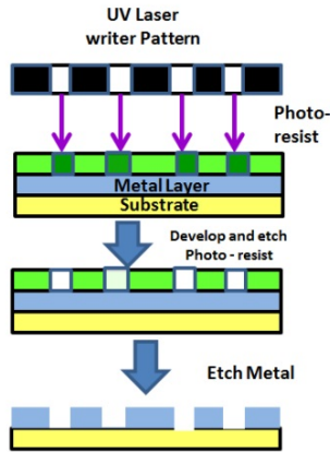
Figure 5. Schematic of the optical sieve fabrication process.
