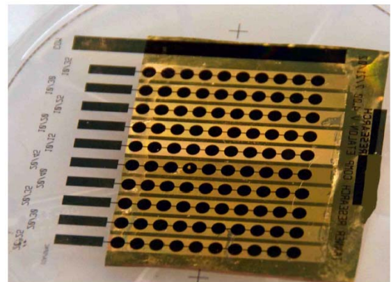
Figure 14 16 x 16 Array of Elastomer Fabry Perot Etalons.
