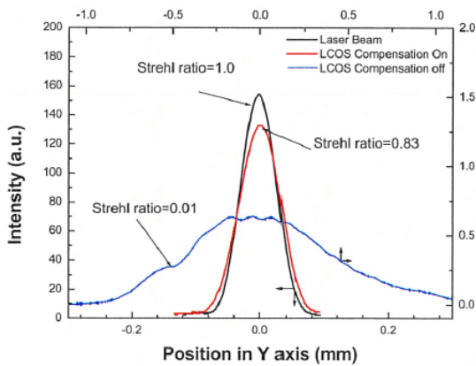
Figure 10. Beam profile of a focused laser beam.
