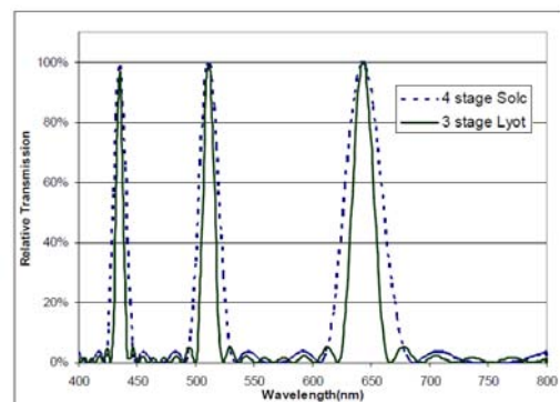
Figure 12. Transmissions of the Lyot and Solc spectral filters.
