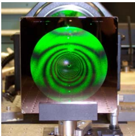
Figure 6. Optical Sieve fabricated at LaRC
