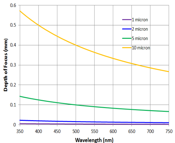
Figure 4. Depth of Focus of Optical Sieve.
