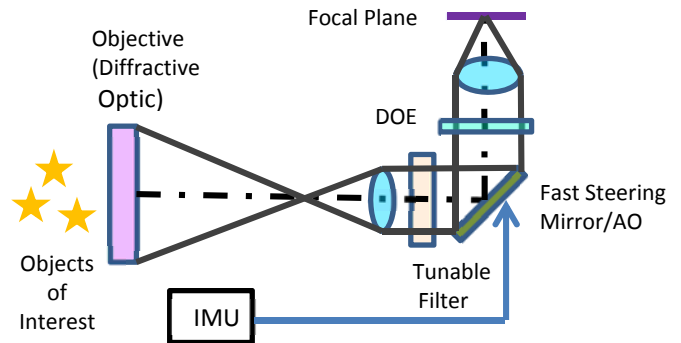
Figure 1. Concept layout of the Ultralight weight Diffractive Optical Telescope System.
