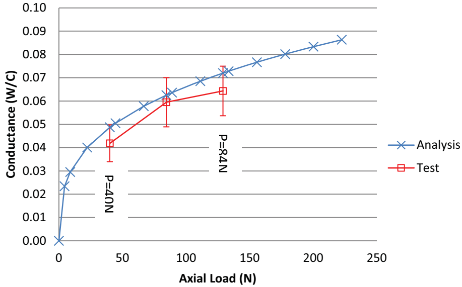
Figure 3.2.1 Theoretical and Experimental Conductance vs. Axial Load for a 28-mm OD Dry Static Steel Bearing
