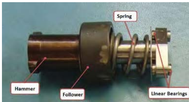
Figure 15. Hammer Sub Assembly
