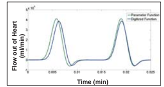
Figure 2: Plot of heart outflow against time for both the digitized function and the functional parameters obtained, as given in [3].
