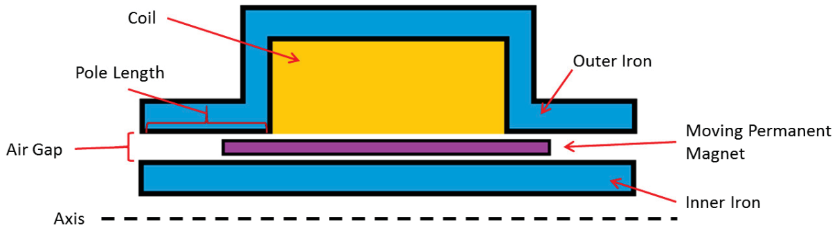
Figure 10.—Linear alternator generic two-dimensional cross section assumed by Sage.
