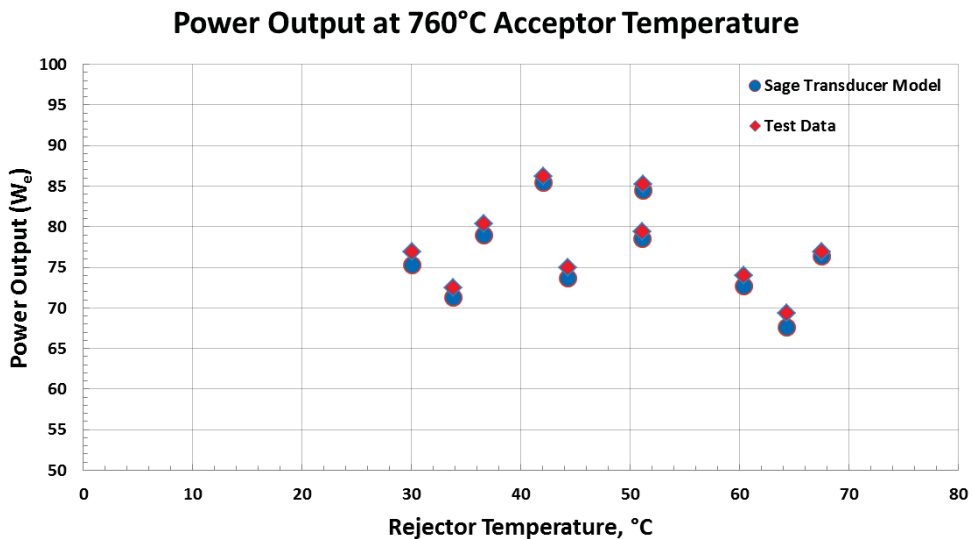
Figure 15.—Sage Advanced Stirling Convertor (ASC) model with transducer alternator; comparison of power output.
