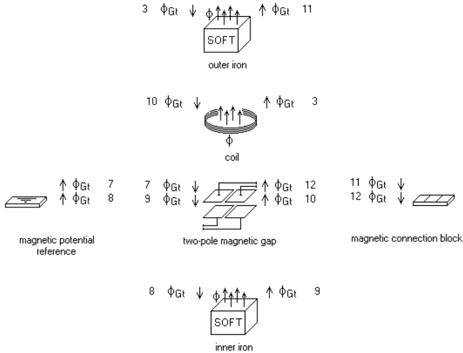
Figure 8.—Sage linear alternator high-level components.
