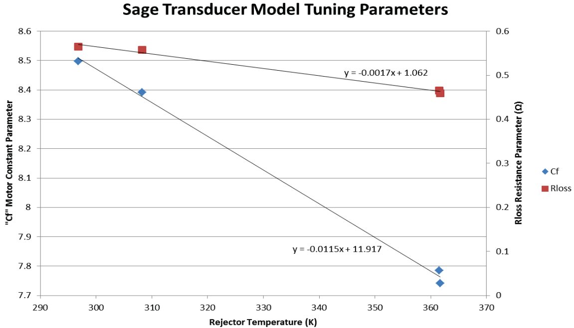
Figure 7.—Transducer tuning parameter value as a function of rejector temperature.
