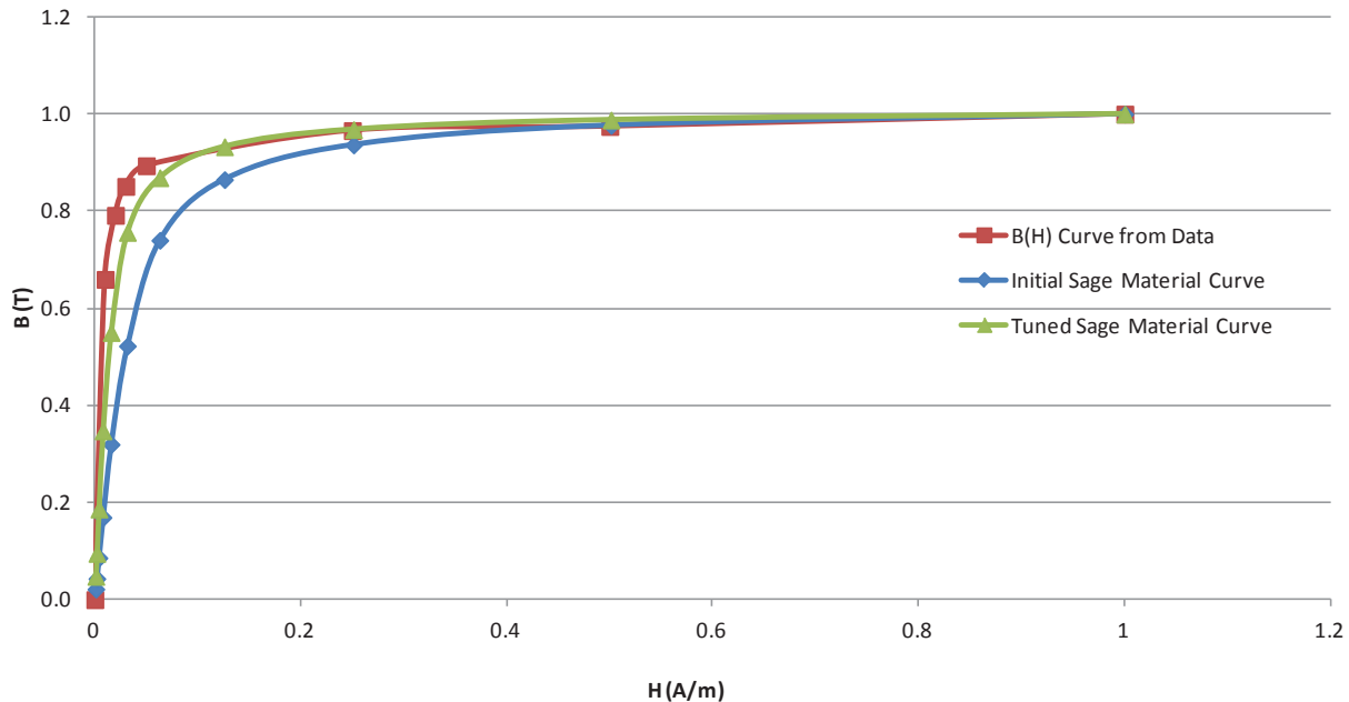
Figure 12.—B(H) curve matching in Sage for ferromagnetic core material.
