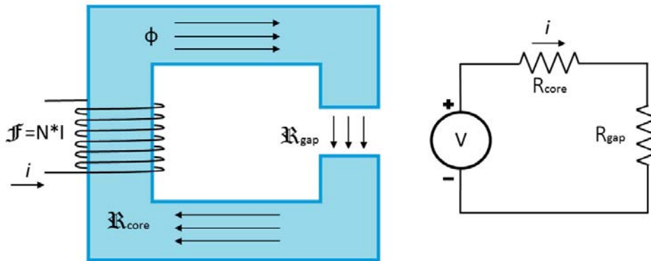
Figure 9.—Magnetic circuit analogy.
