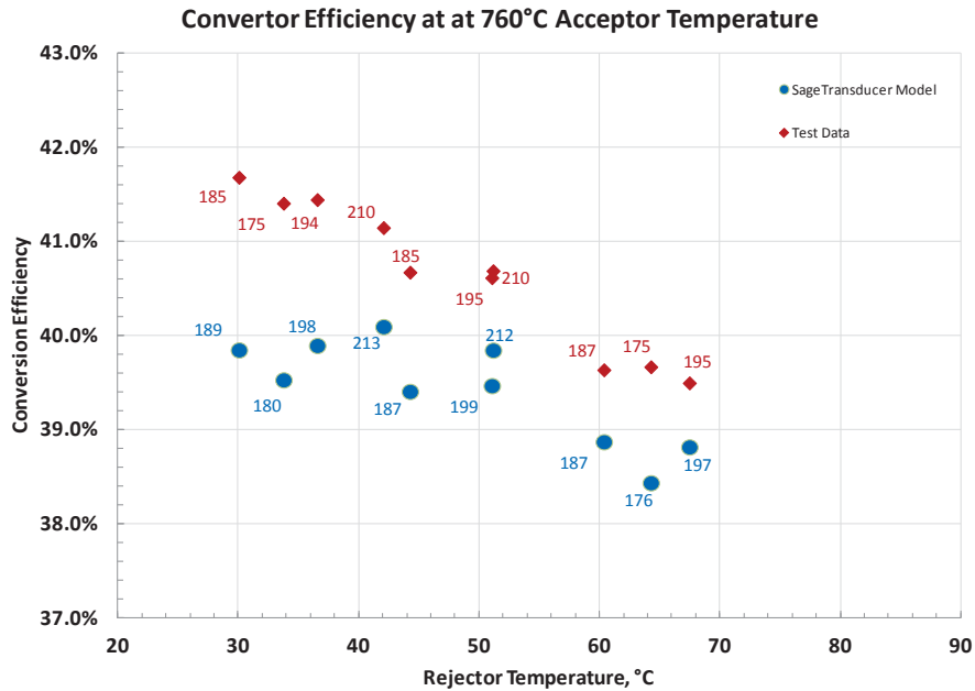
Figure 14.—Sage Advanced Stirling Convertor (ASC) model with transducer alternator; comparison of convertor efficiency.
