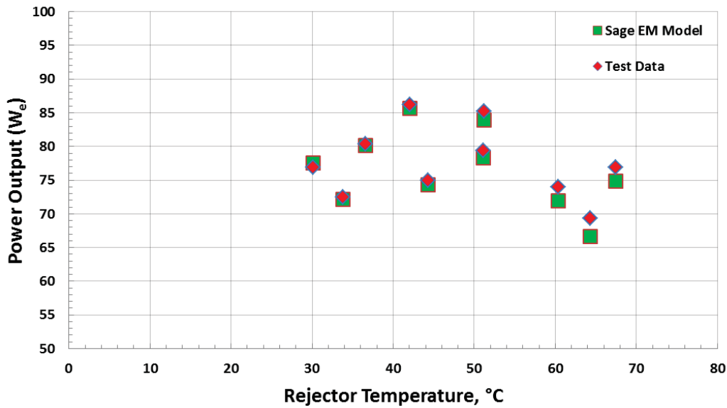
Figure 17.—Sage Advanced Stirling Converter (ASC) model with electromagnetic (EM) alternator; comparison of power output.
