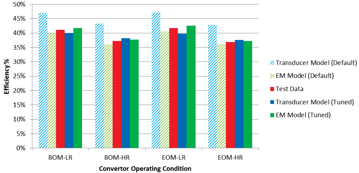
Figure 18.—Sage alternator model convertor efficiency comparison.
