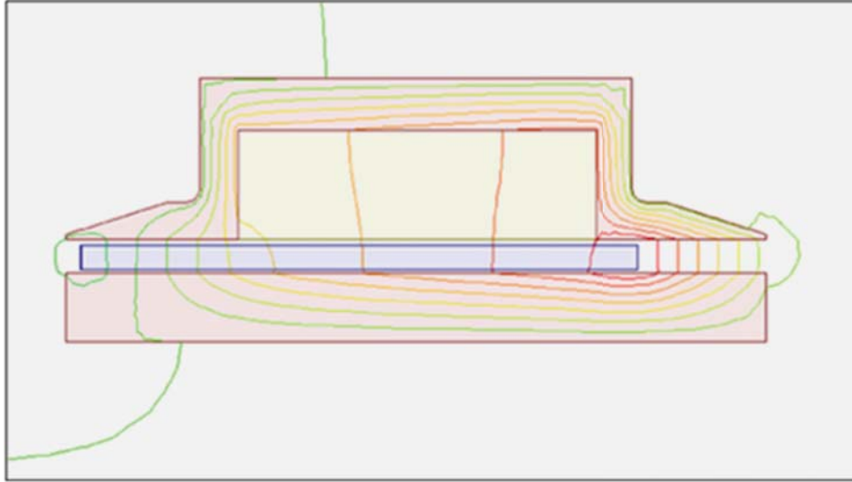
Figure 13.—Two-dimensional magnetic flux plot of a linear alternator.
