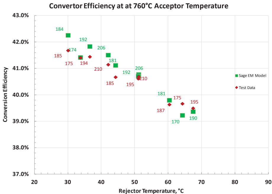
Figure 16.—Sage Advanced Stirling Converter (ASC) model with electromagnetic (EM) alternator; comparison of converter efficiency.
