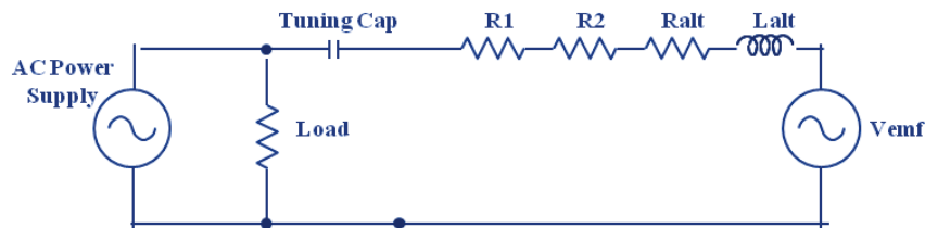
Figure 5.—Circuit diagram of the linear alternator and alternating current (ac) bus controller.
