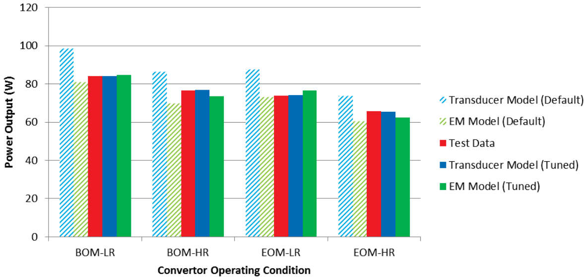
Figure 19.—Sage alternator model power output comparison.
