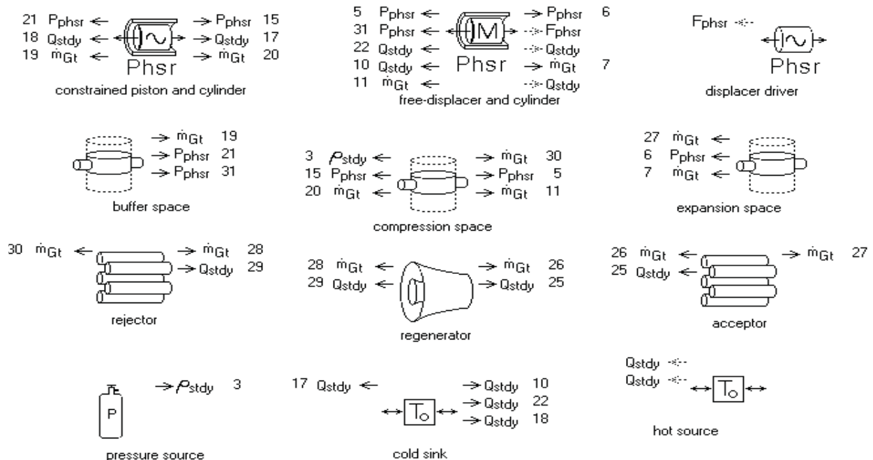
Figure 2.—Sage Stirling engine model.
