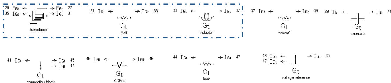
Figure 6.—Linear alternator circuit model in Sage using the transducer component. Outlined are the main linear alternator model components.
