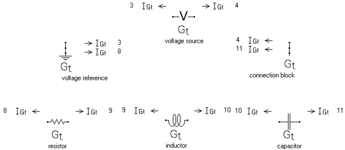
Figure 3.—RLC circuit model in Sage example.
