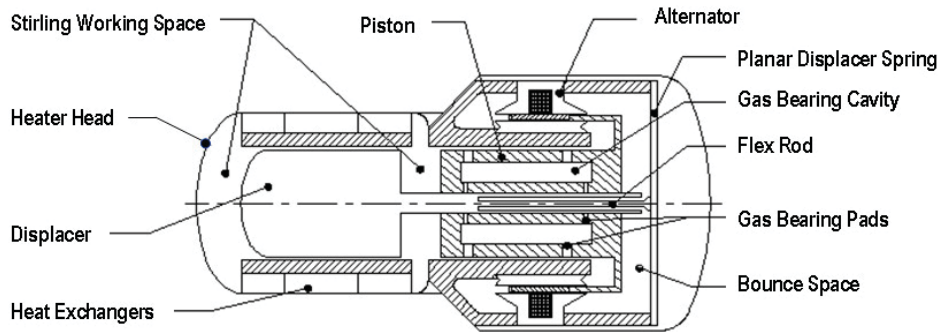
Figure 1.—Advanced Stirling Converter (ASC) cross section layout.
