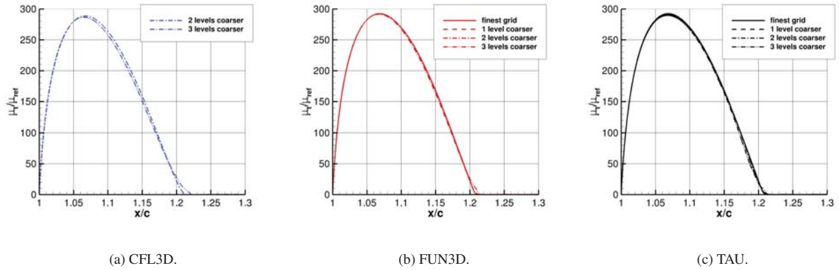
Figure 35. Eddy-viscosity variation behind the trailing edge along the line z = 0 .
