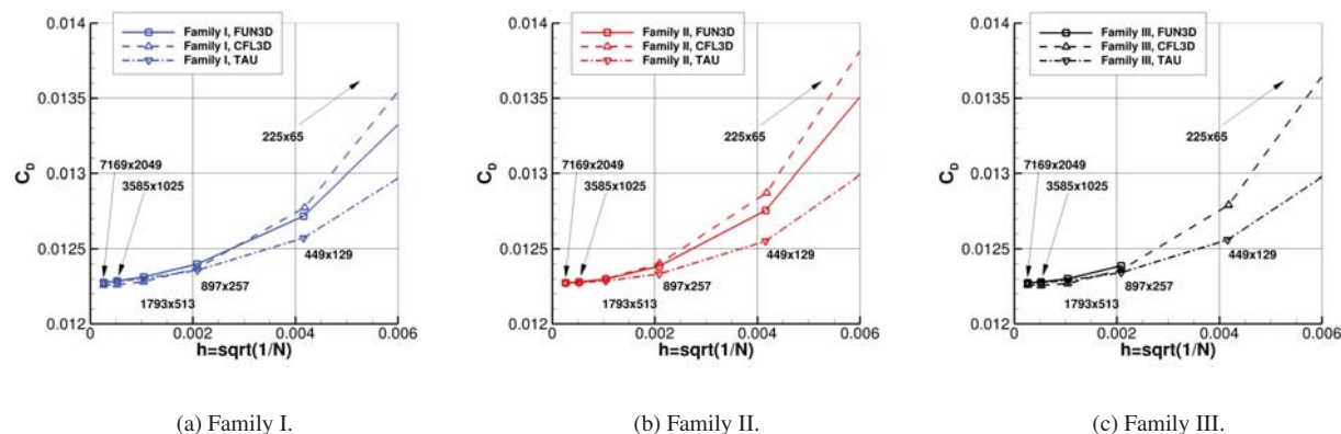
Figure 4. NACA 0012: Grid convergence of the total drag coefficient ( C_D ).
