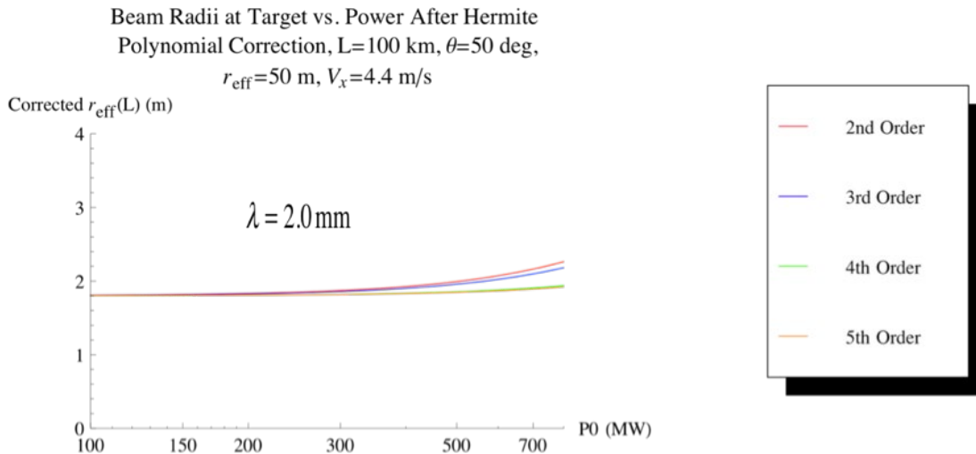
Figure 15.—Beam radius (in m) at target versus power (in MW) for a 5 m for various orders of phase correction.
