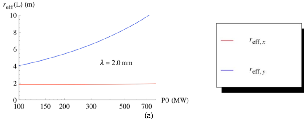
Induced Beam Displacement vs. Power, L=120 km, \theta=90 deg, r_{\text{eff}}=50 m, V_x=4.4 m/s
